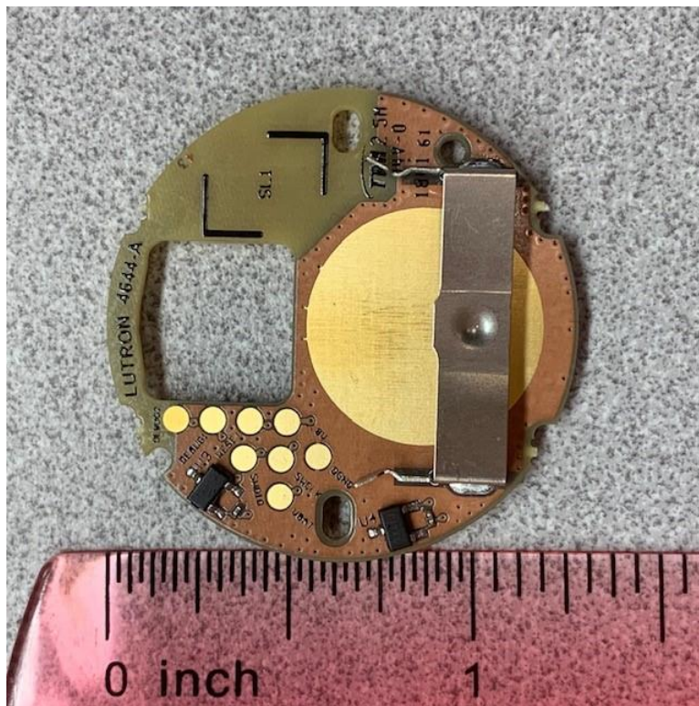
Z3-1BRL Board Rear
