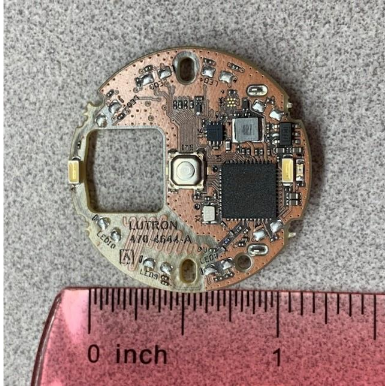
Z3-1BRL Board Front
