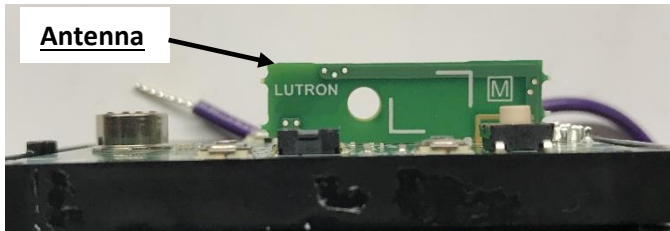
Antenna board affixed to sensor board
