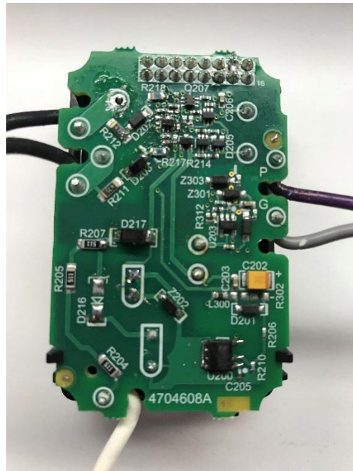
8SD Power board back
