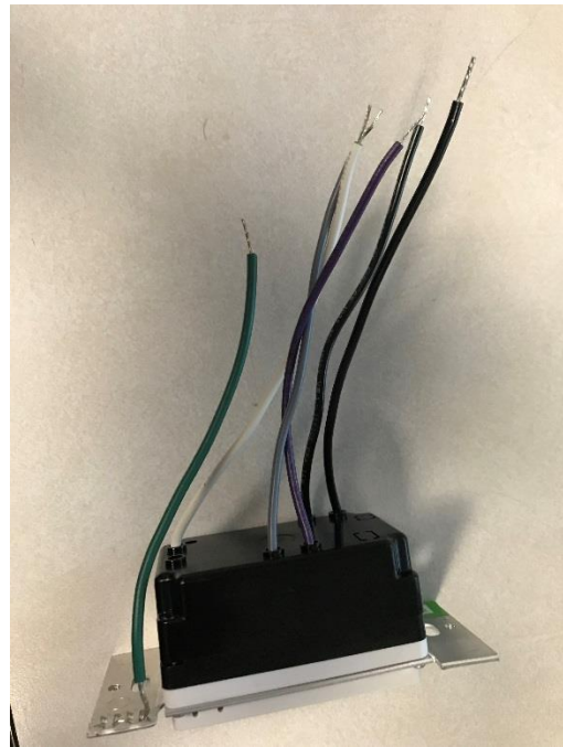
8SD Side/Rear view
