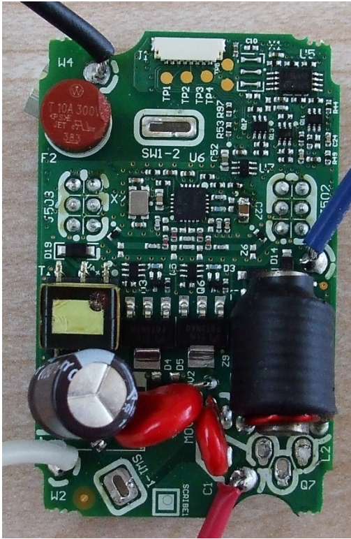
GT-RF2 Back of Power Board
