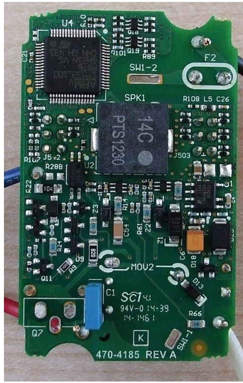
GT-RF Front of Power Board
