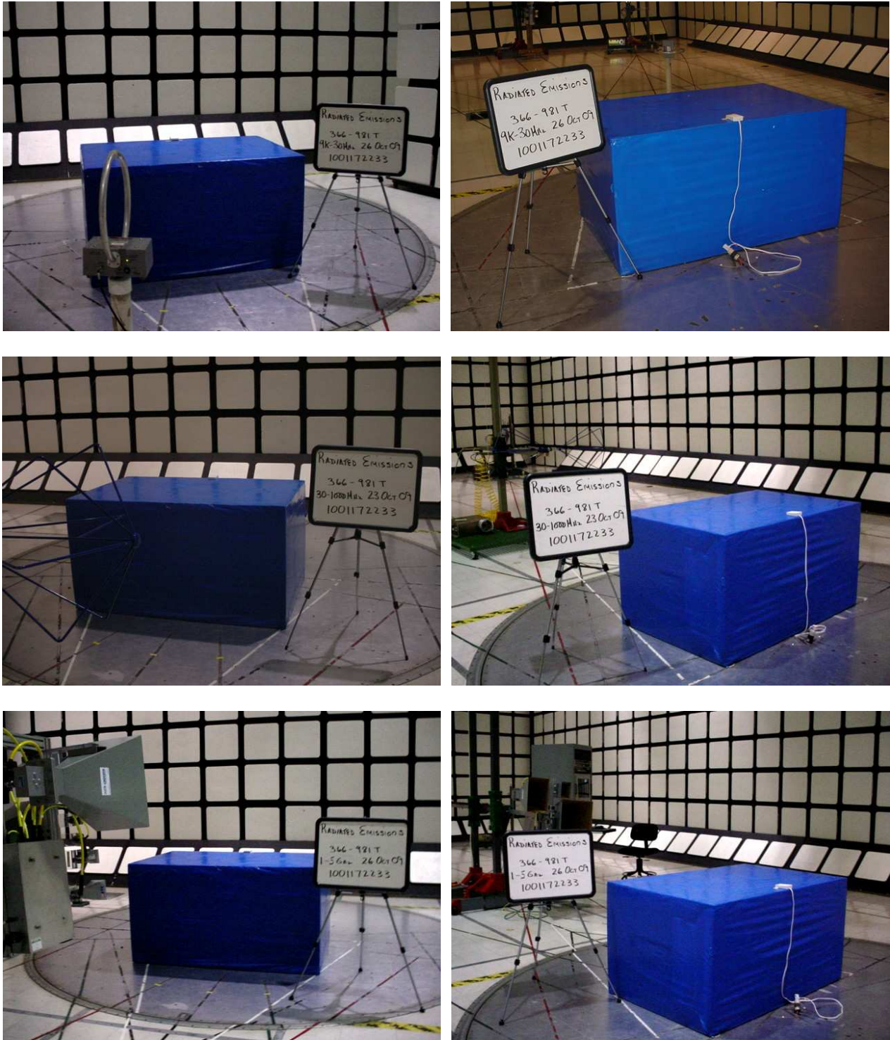
Figure 13 Test setup for Radiated Emissions
