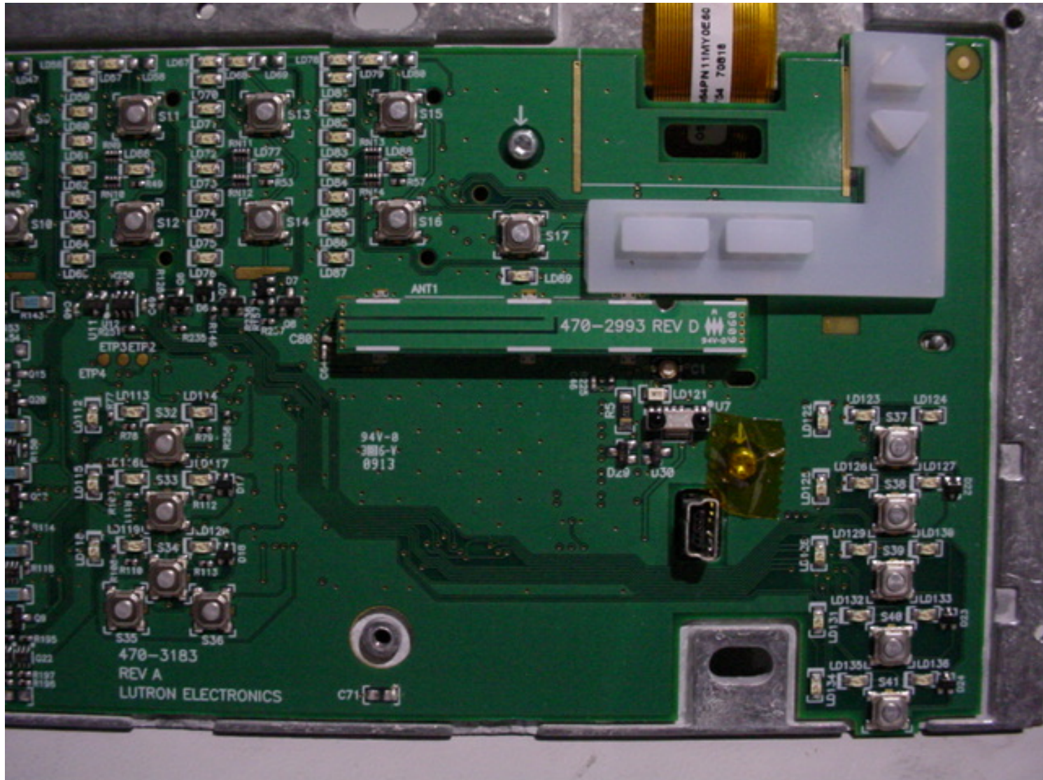
Front PCB (Right Side)
