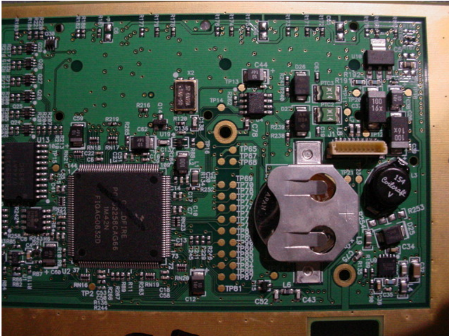
Rear PCB (Right Side)
