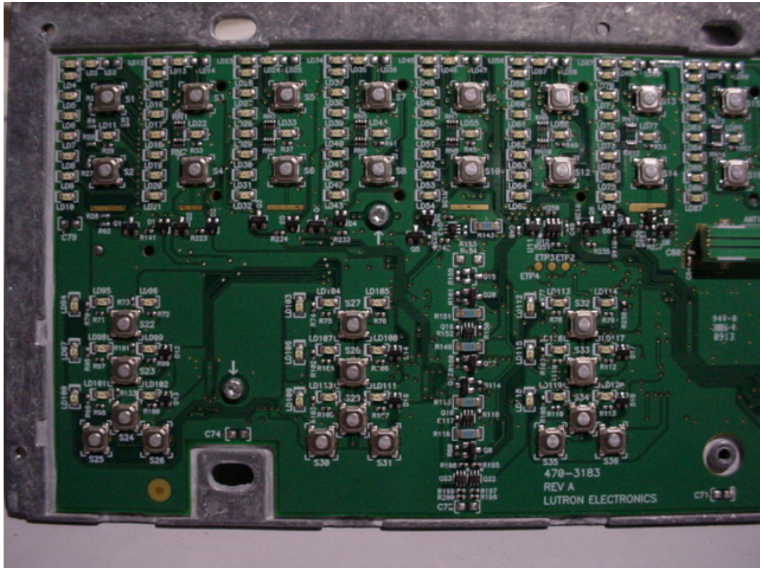
Front PCB (Left Side)
