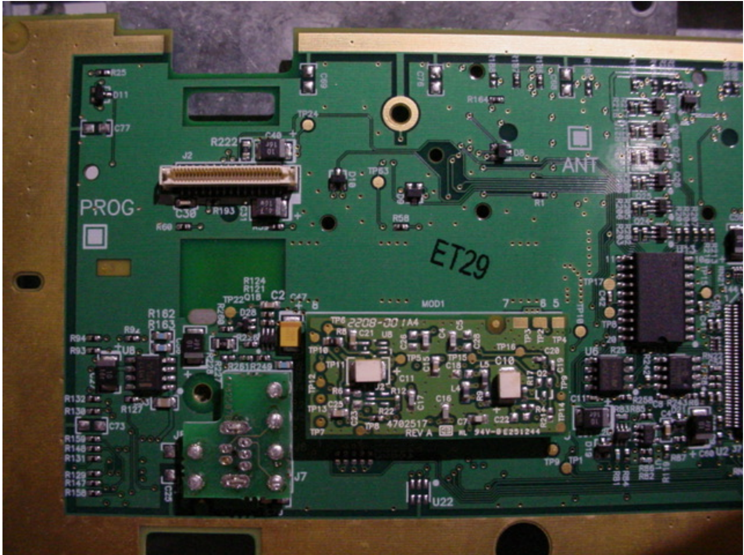
Rear PCB (Left Side)
