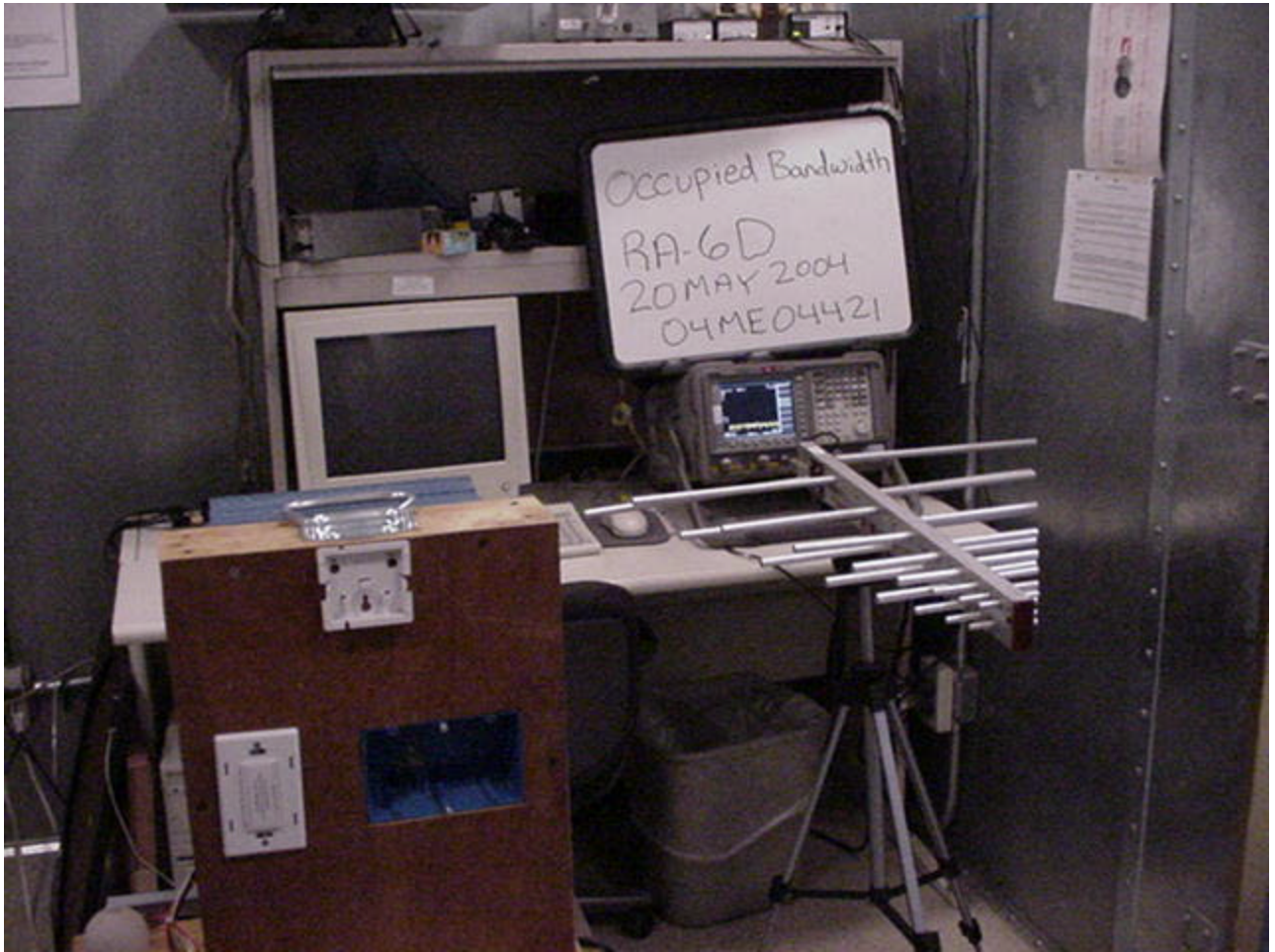
Occupied Bandwidth Test Set-Up
