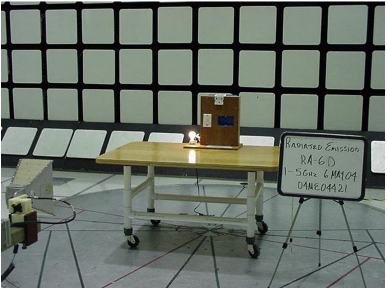
Radiated Emission Test Set-up Front View 1-5GHz
