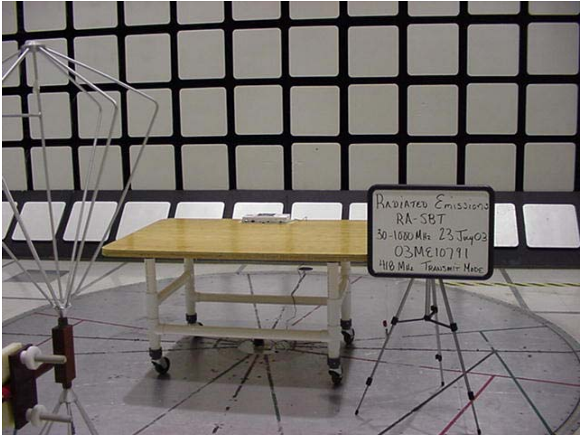
Radiated Emission Test Set-Up 30-1000MHz Front View
