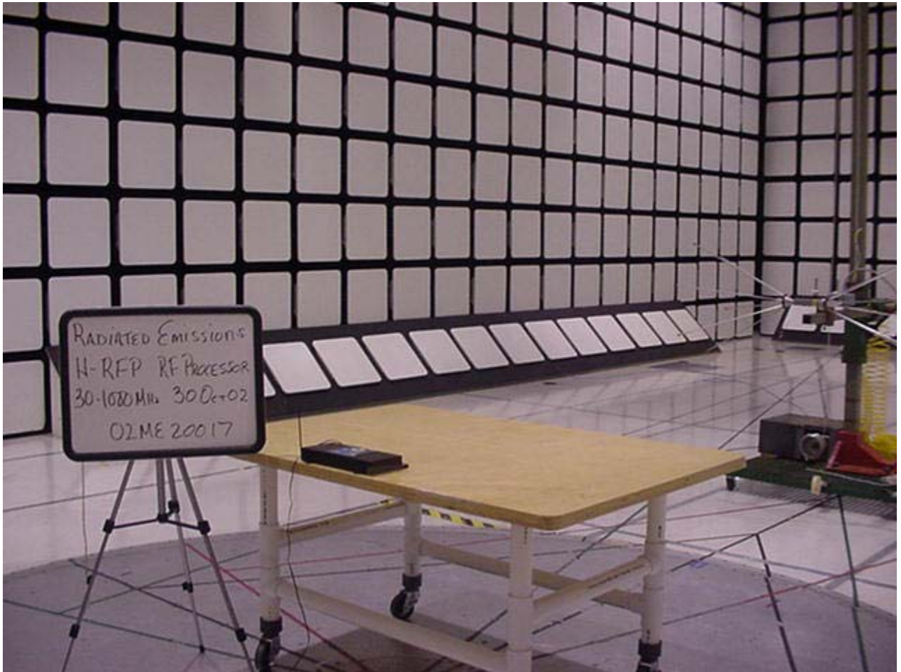
Radiated Emissions Test Set-Up 30-1000MHz Rear View
