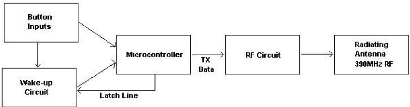
Transmitter Block Diagram
