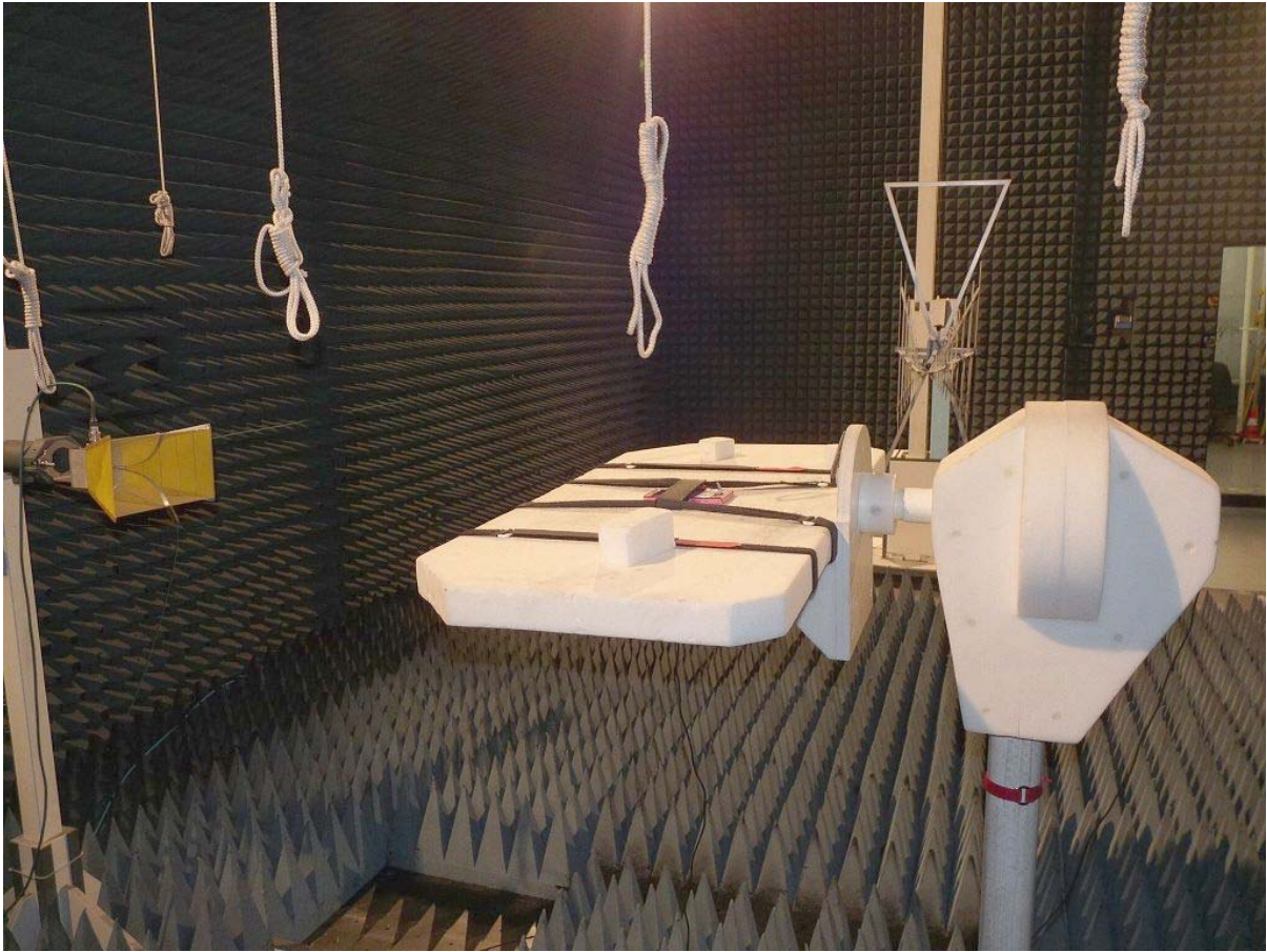
Photo 3: Test setup for radiated measurements (Enclosure, 1-18 GHz $15, 30 MHz – 20 GHz $24)
