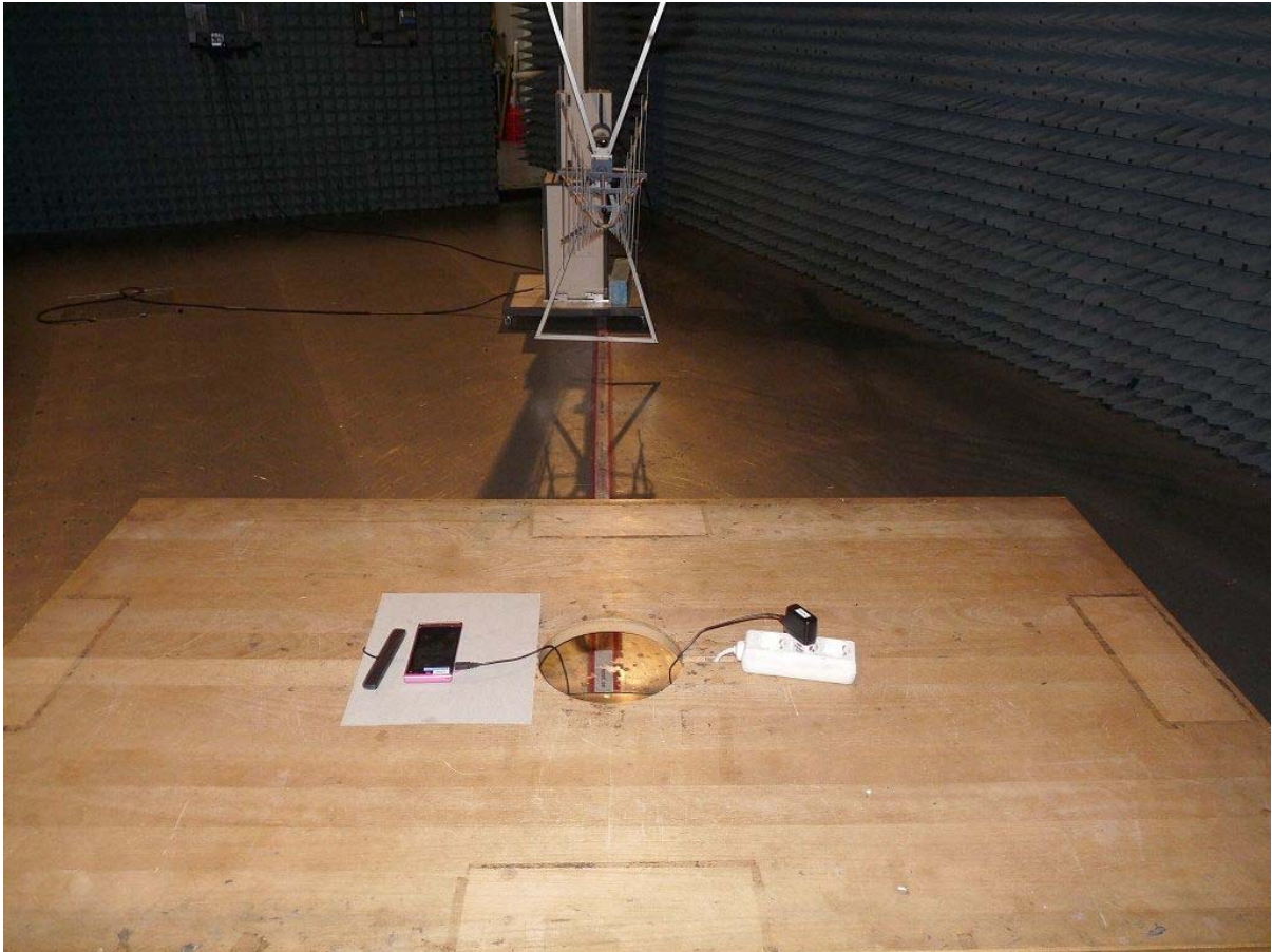
Photo 2: Test setup for radiated measurements (Enclosure, 30 MHz to 1 GHz, $15)
