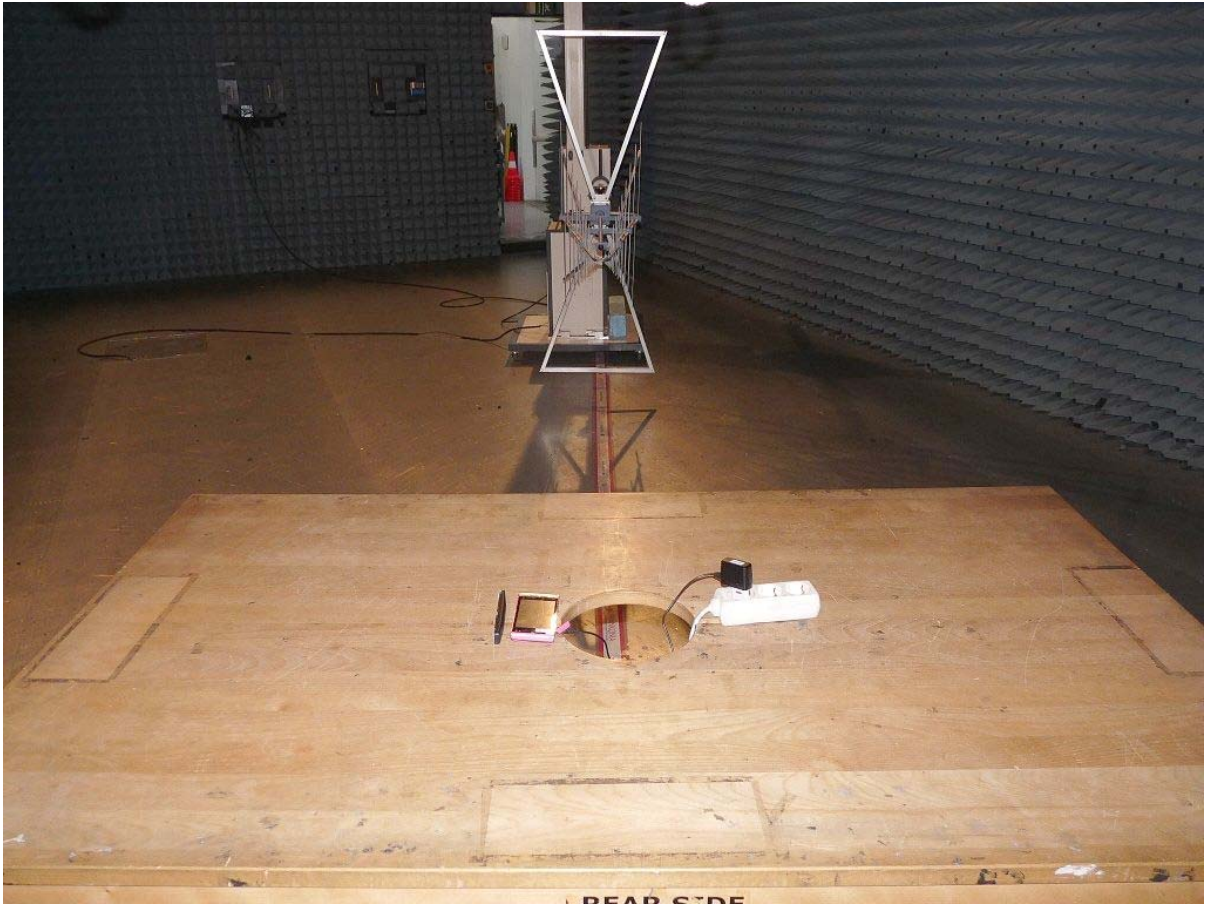
Photo 7: Test setup for radiated measurements (AC Port (power line), EUT supplied by AC/DC adapter)
