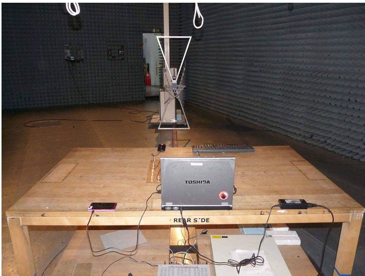
Photo 8: Test setup for radiated measurements (computer peripheral setup, EUT supplied by USB-cable from computer)
