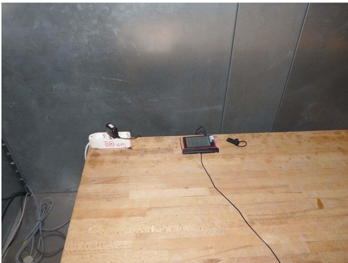
Photo 5: Test setup for conducted measurements (AC Port (power line), EUT supplied by AC/DC adapter)
