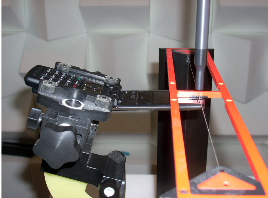
Figure 17-1 Ear Reference Point HAC Phantom Alignment
