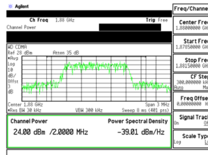
Figure 8-2 Wireless Device Modulated Signal
