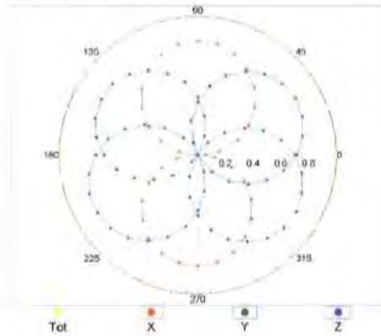
f=600 MHz,TEM
