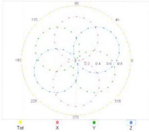
f=600 MHz,TEM
