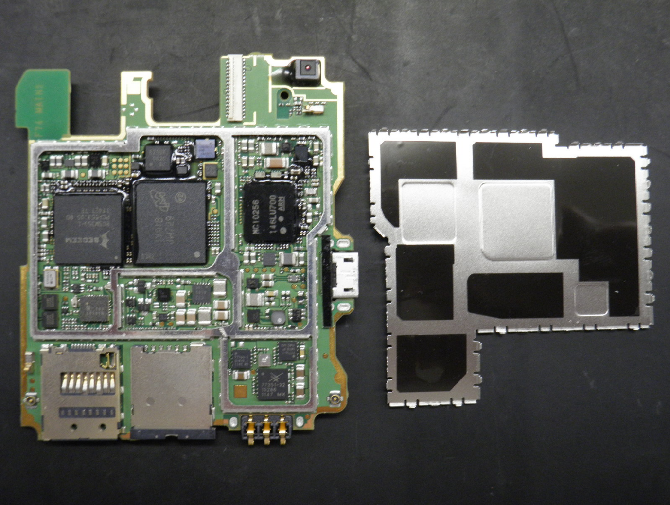
MAIN PCB L1 without Shield
