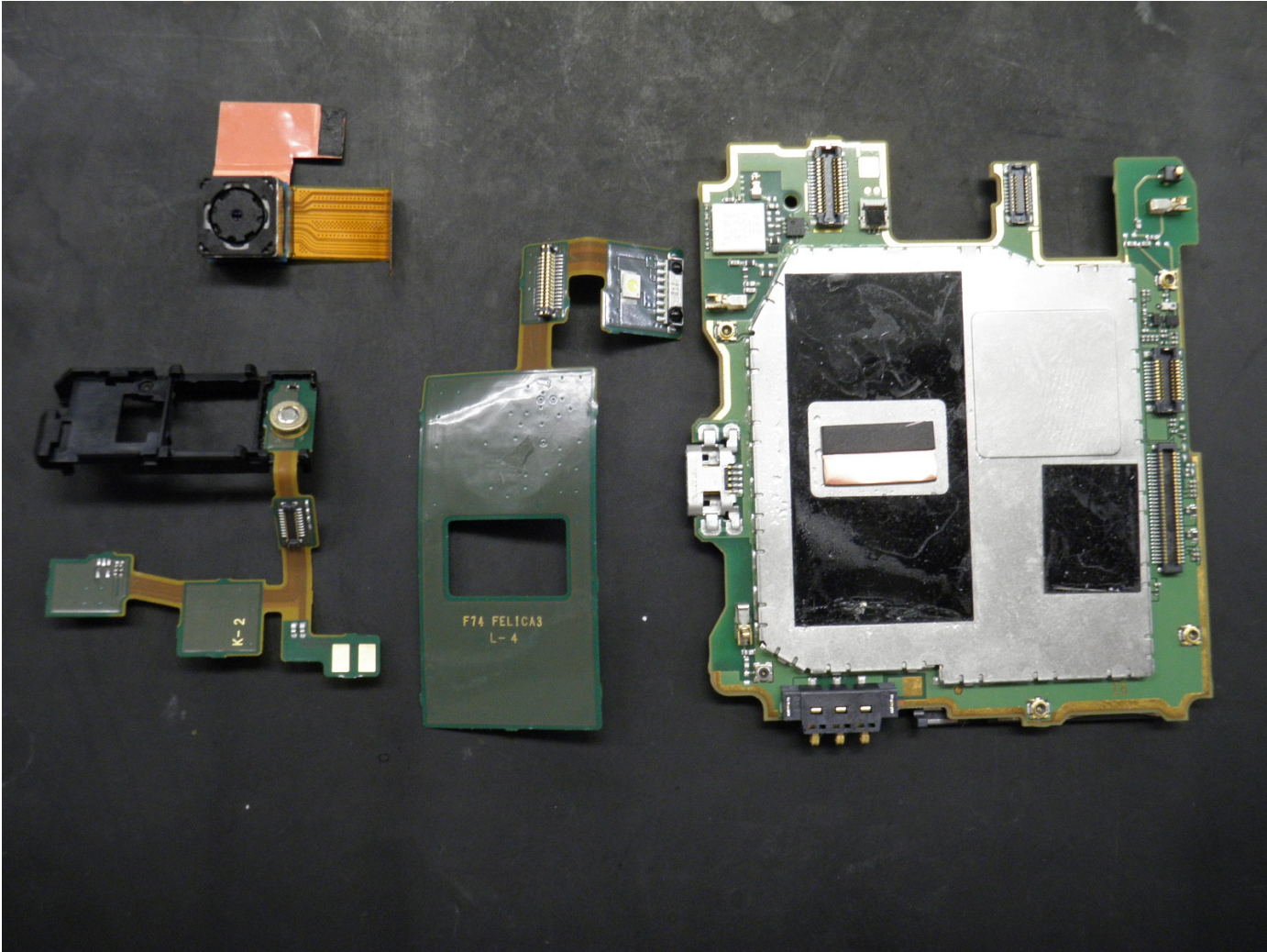
SUB PCB / FeliCa FPC / CAMERA FPC / MAIN PCB
