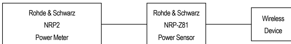
Figure 10.4 Power Measurement Setup for Bandwidths < 50 MHz
