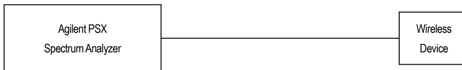
Figure 10.5 Power Measurement Setup for Bandwidths > 50 MHz
