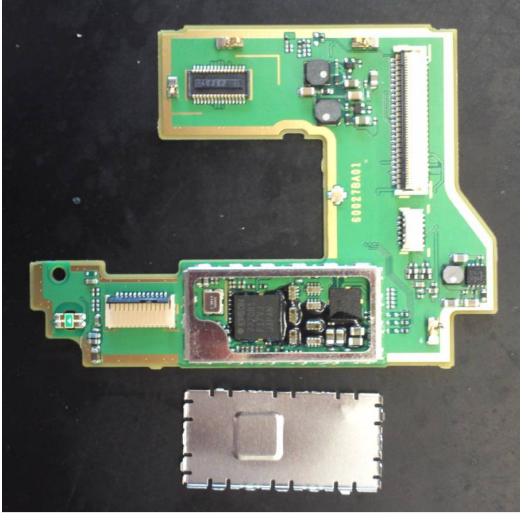
LCD PCB L1 without Shield
