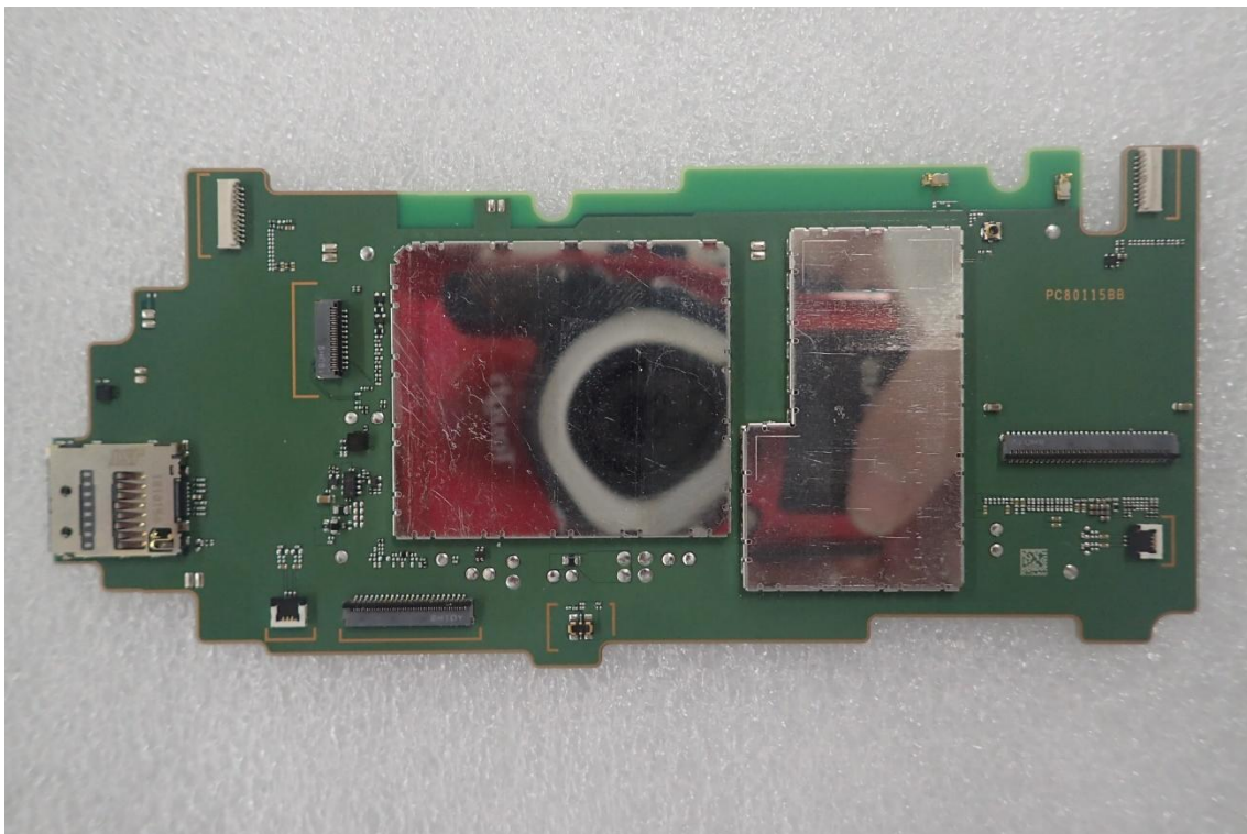
Main PCB front
