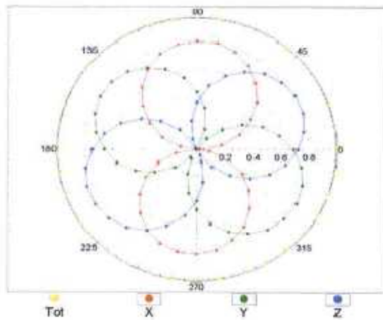
f=600 MHz,TEM
