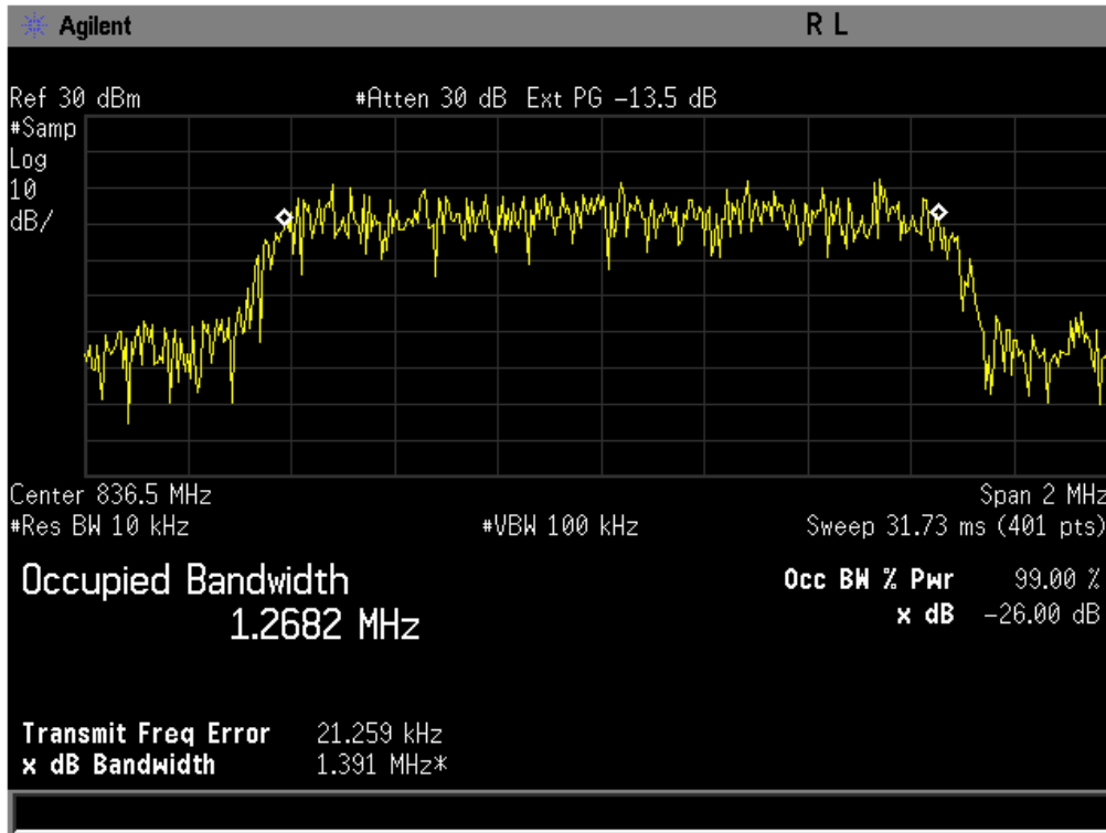
Figure 8-1 CDMA 800 @ CH 383
