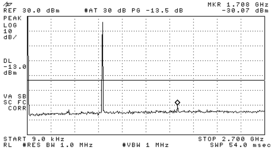
Figure 9-3a CDMA 800 – Conducted Spurious Emission (CH 777)
