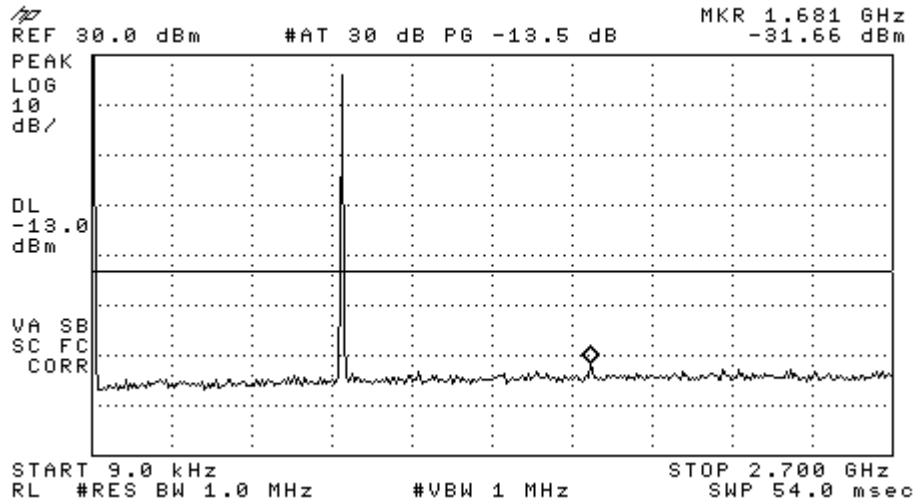
Figure 9-2a CDMA 800 – Conducted Spurious Emission (CH 383)
