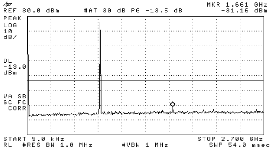
Figure 9-1a CDMA 800 – Conducted Spurious Emission (CH 1013)
