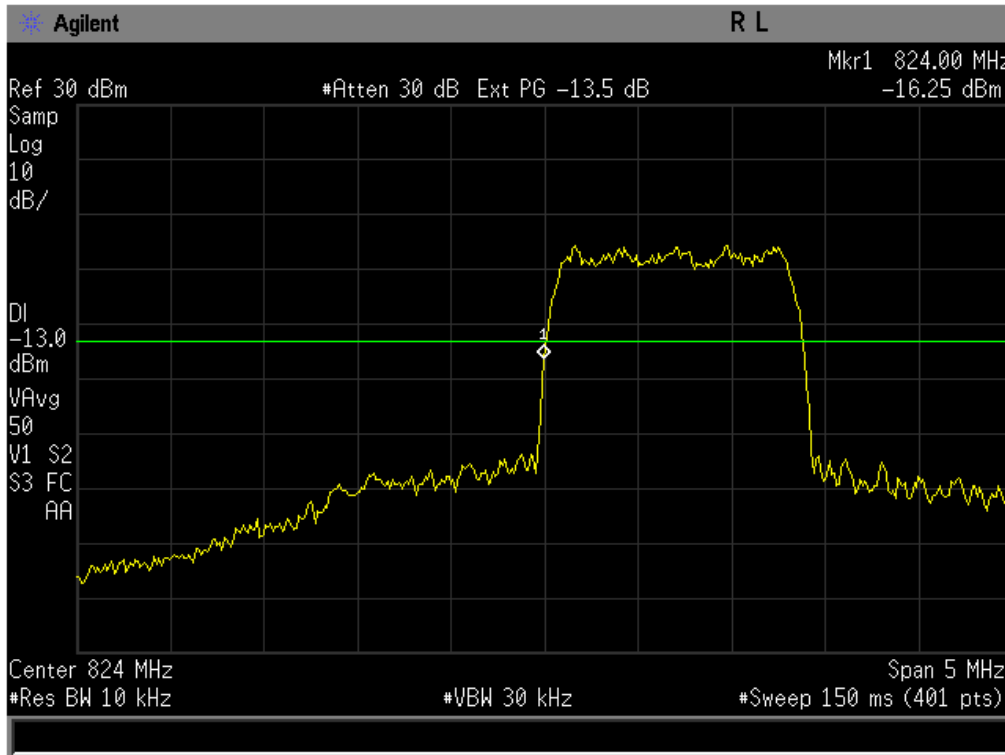
Figure 8-2 CDMA 800 Lower Band Edge @ CH 1013
