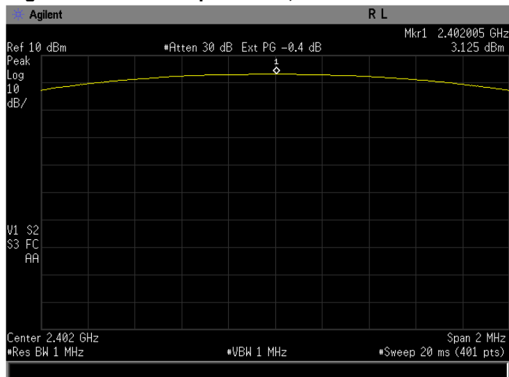
Figure 5-1b: Peak Output Power, EDR D8PSK Channel 0.
