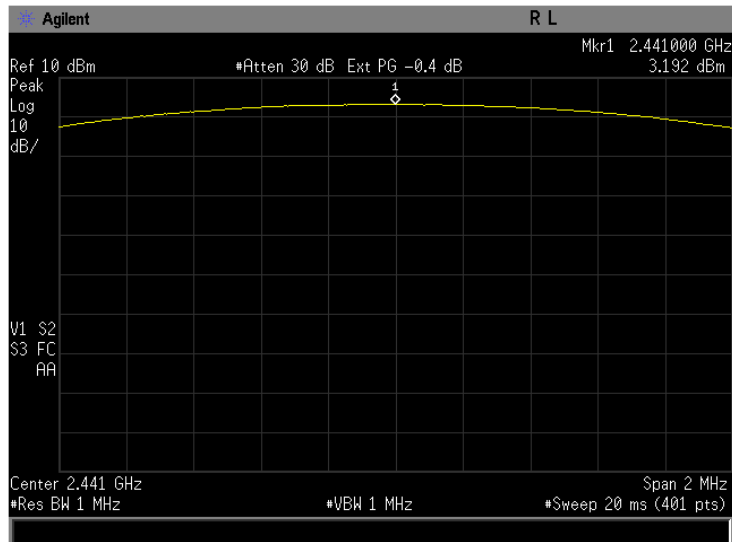
Figure 5-2b: Peak Output Power, EDR D8PSK Channel 39.
