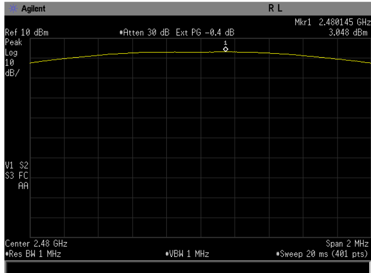
Figure 5-3a: Peak Output Power, EDR DQPSK Channel 78.
