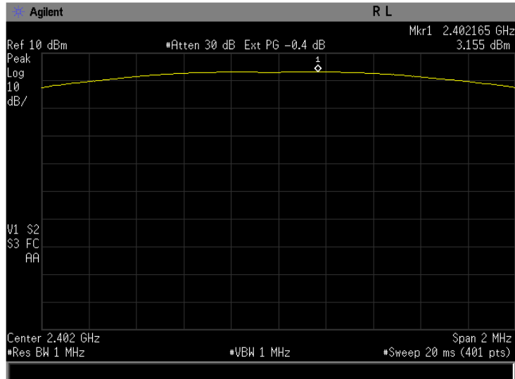
Figure 5-1a: Peak Output Power, EDR DQPSK Channel 0.
