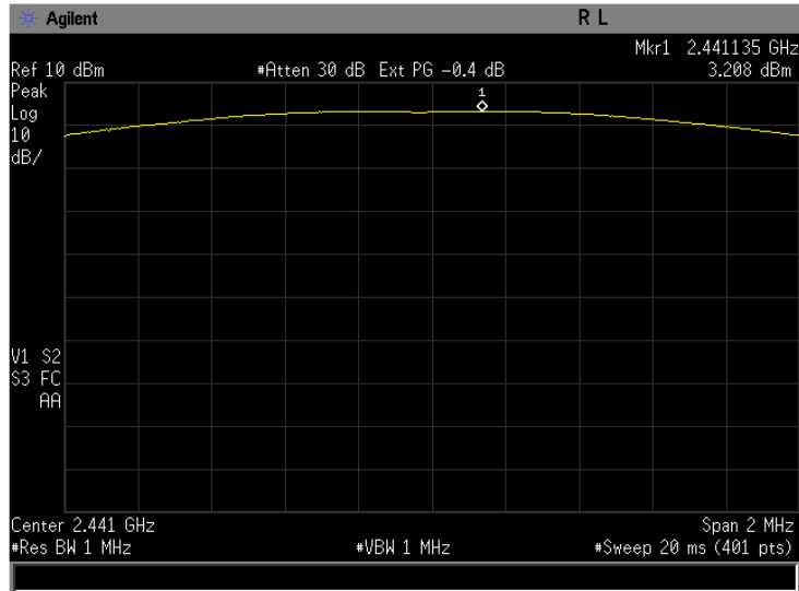
Figure 5-2a: Peak Output Power, EDR DQPSK Channel 39.
