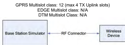
Figure 8.1 Power Measurement Setup
