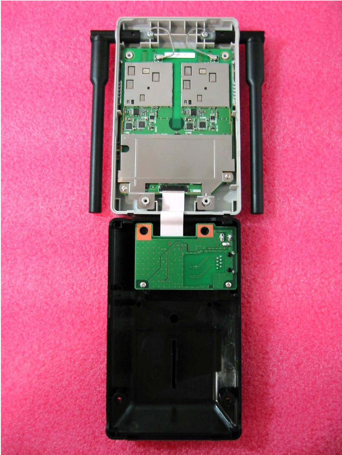
Main + I/F Board
