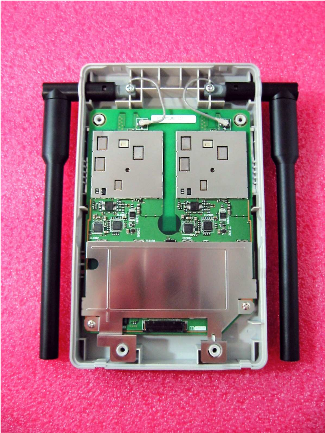
Main Board
