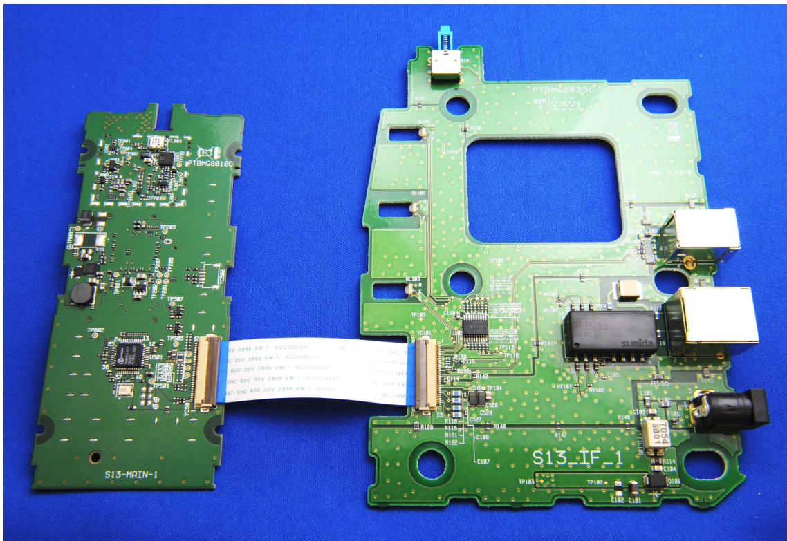
Main Board – I/F Board
