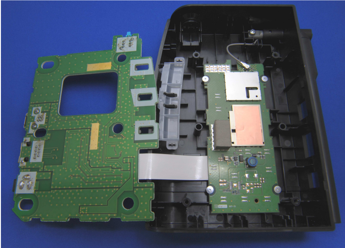
I/F Board – Main Board w/ Case
