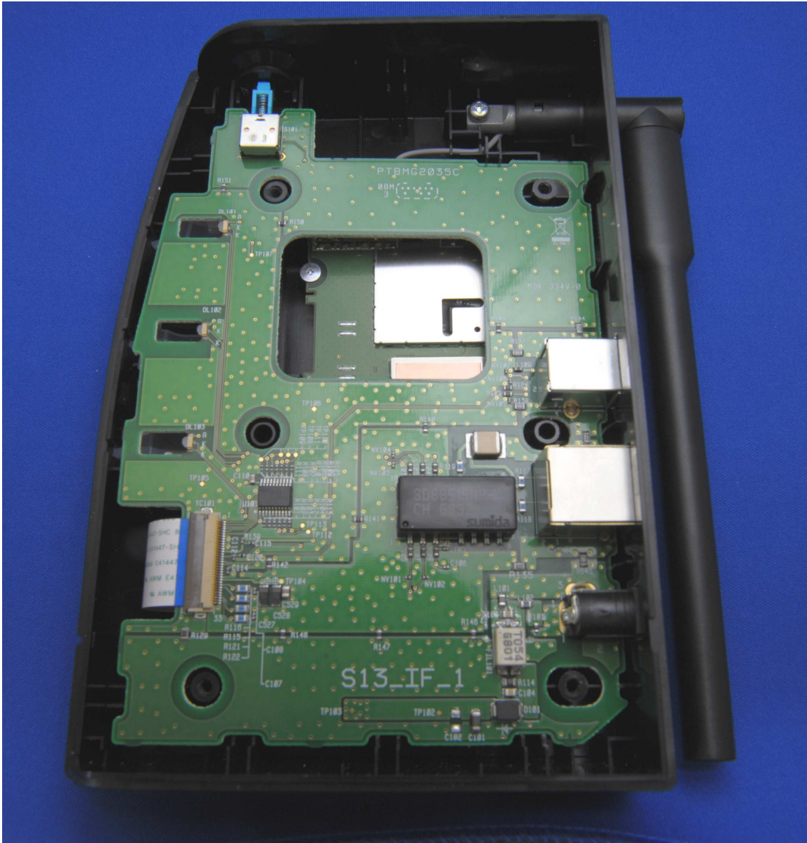
I/F Board – Main Board w/ Case (Built-In)
