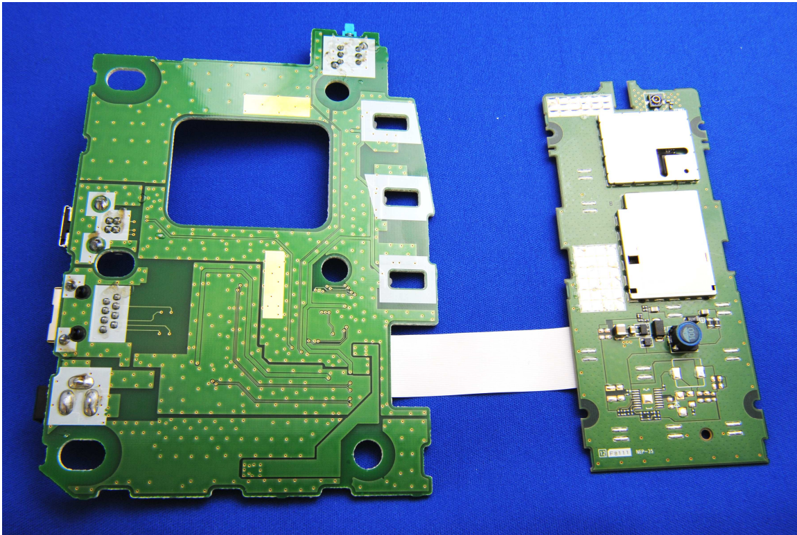
I/F Board – Main Board (Back)
