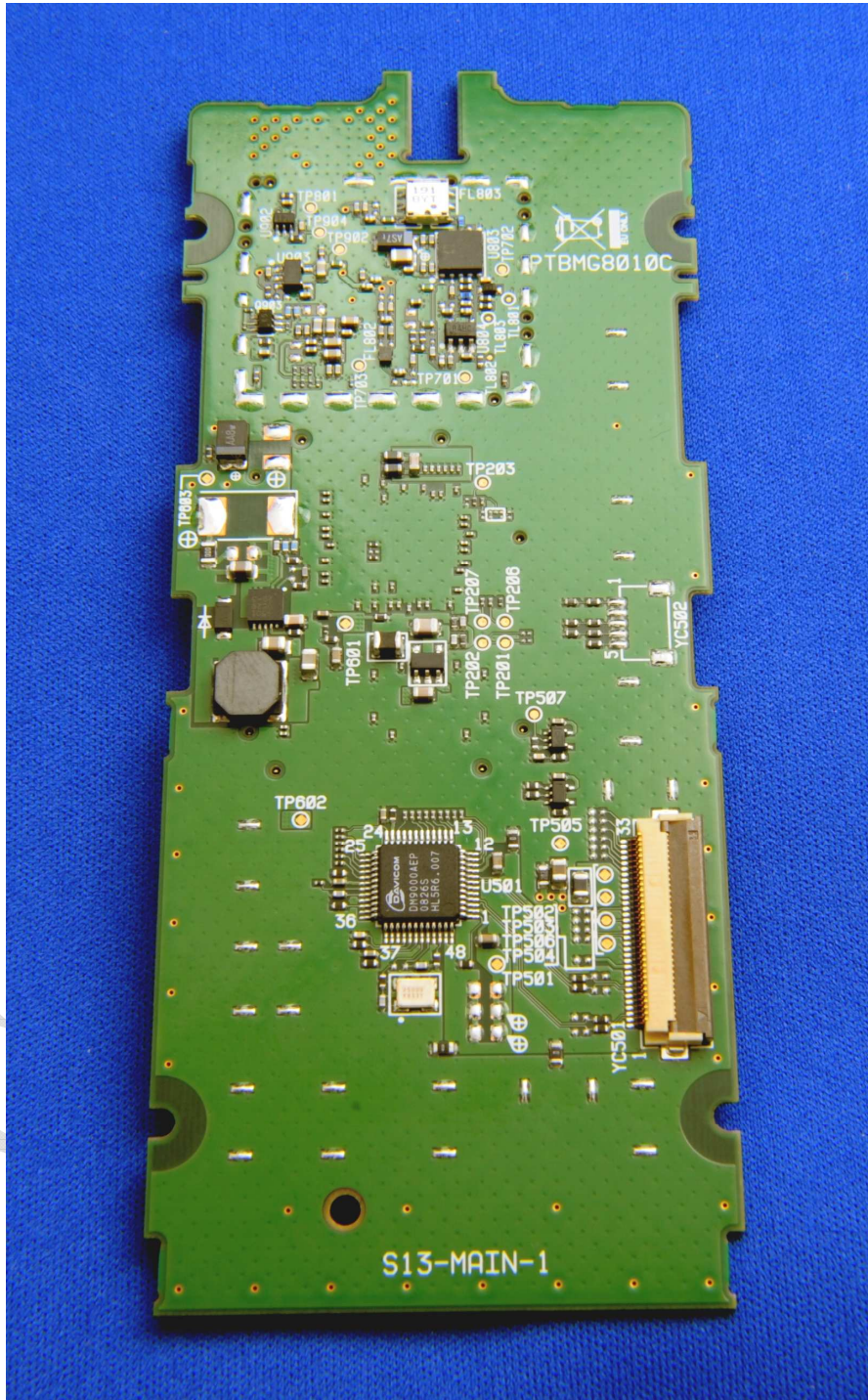
Main Board – L1
