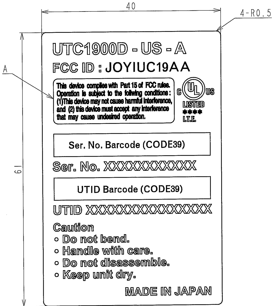
SCALE=2/1 Detail of SERIAL NO. PLATE
