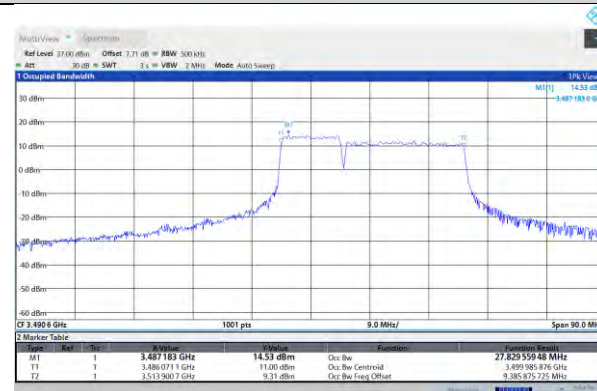
42-42-10MHz-20MHz-16QAM-16QAM-42145-42289- 50RB#0-100RB#0
