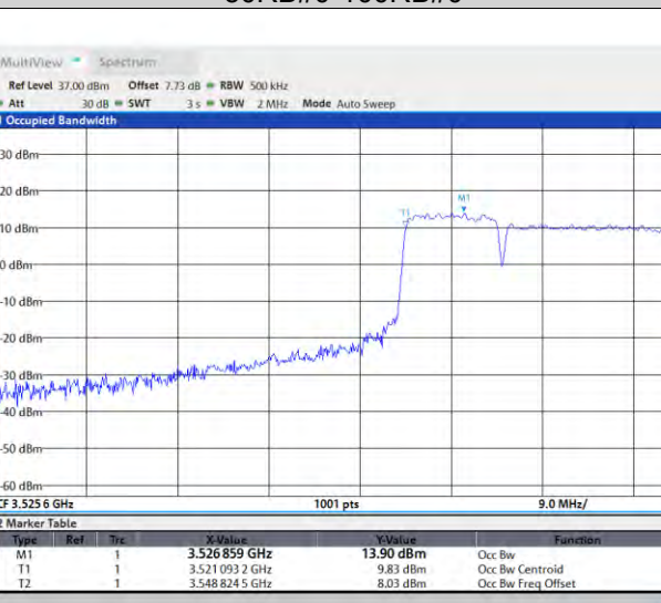
42-42-10MHz-20MHz-64QAM-64QAM-42496-42640- 50RB#0-100RB#0
