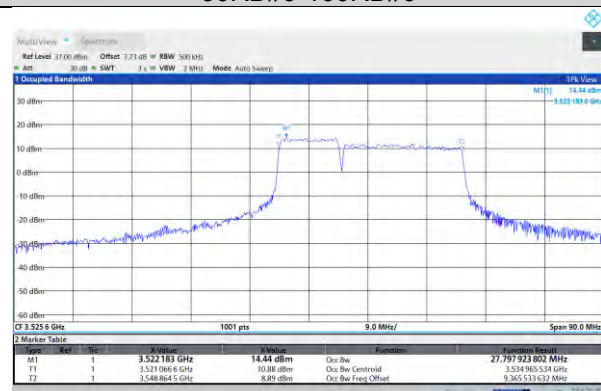
42-42-10MHz-20MHz-16QAM-16QAM-42496-42640- 50RB#0-100RB#0
