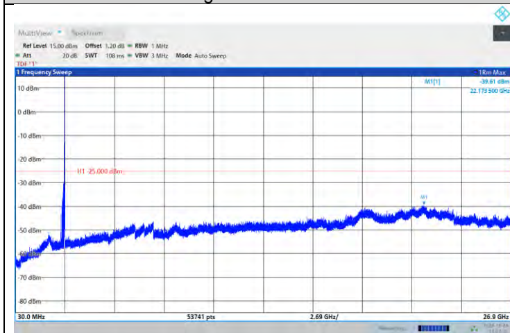
Band41-20MHz-QPSK-40620-1RB#0- Range:30~26900MHz
