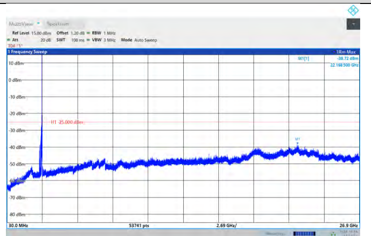
Band41-20MHz-16QAM-40620-1RB#0-Range:30~26900MHz
