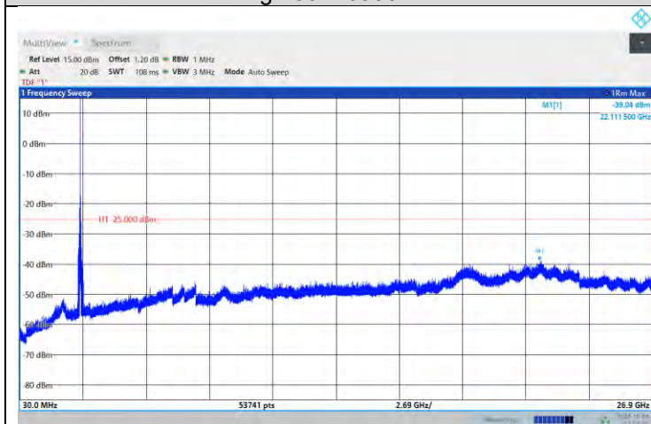
Band41-20MHz-16QAM-39750-1RB#0- Range:30~26900MHz
