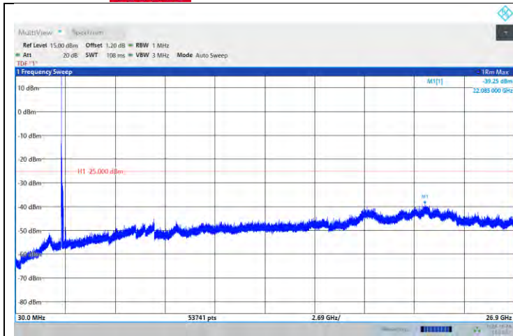
Band41-10MHz-16QAM-41540-1RB#0- Range:30~26900MHz
