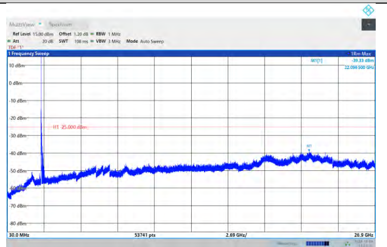
Band41-20MHz-QPSK-41490-1RB#0-Range:30~26900MHz
