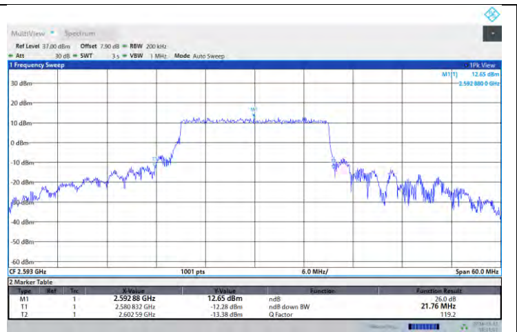
Band41-20MHz-64QAM-39750-100RB#0
