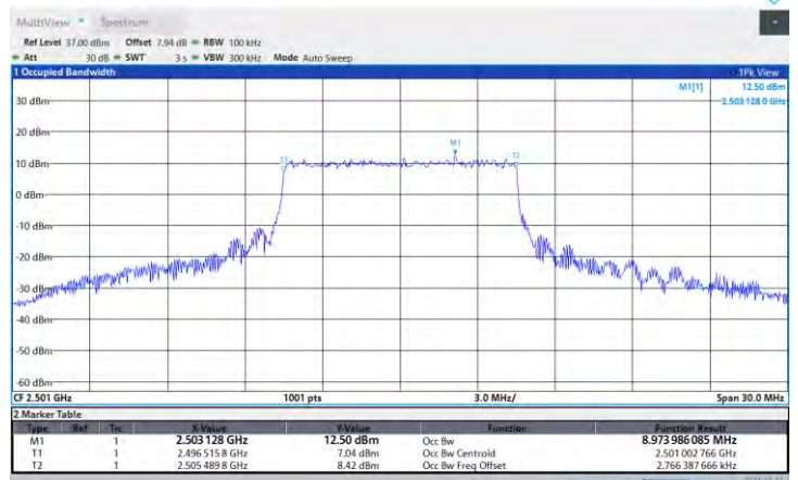
Band41-10MHz-64QAM-41540-50RB#0
