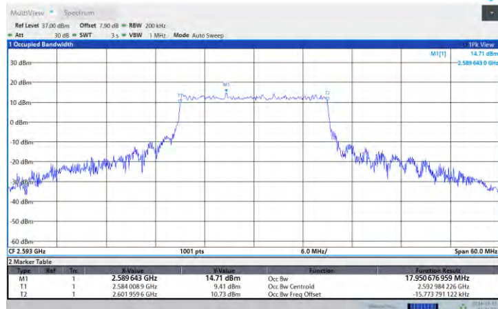
Band41-20MHz-16QAM-39750-100RB#0
