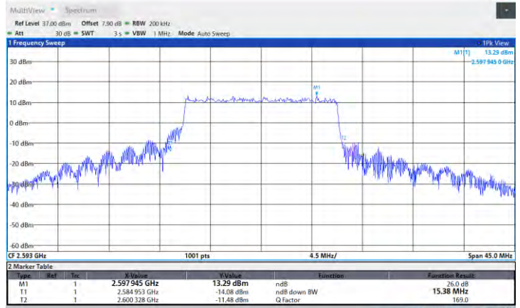
Band41-20MHz-QPSK-39750-100RB#0
