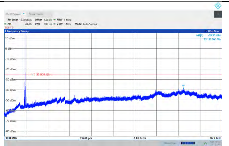
Band41-10MHz-64QAM-39700-1RB#0-Range:30~26900MHz
