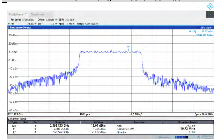
Band41-20MHz-64QAM-40620-100RB#0
