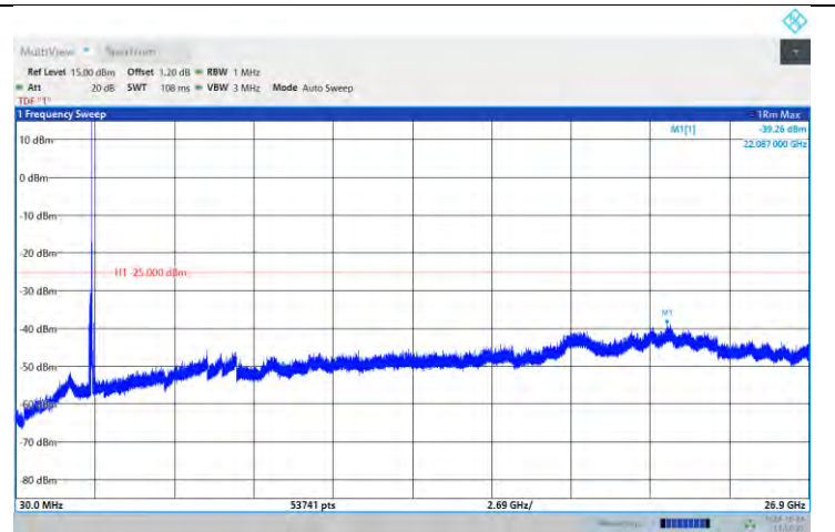
Band41-20MHz-QPSK-39750-1RB#0-Range:30~26900MHz
