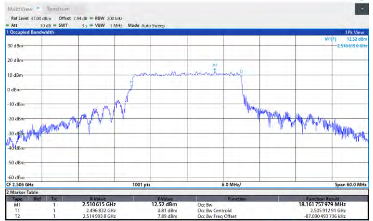
Band41-20MHz-64QAM-41490-100RB#0
