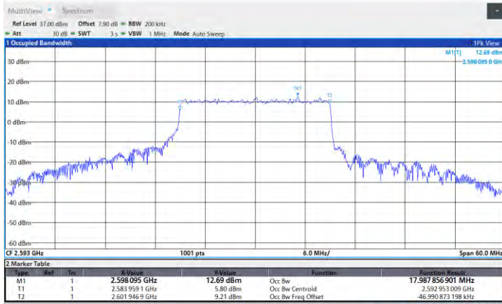
Band41-20MHz-64QAM-40620-100RB#0
