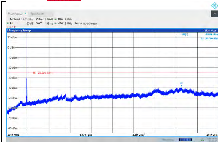
Band41-15MHz-64QAM-41515-1RB#0- Range:30~26900MHz
