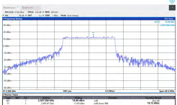
Band41-20MHz-QPSK-41490-100RB#0
