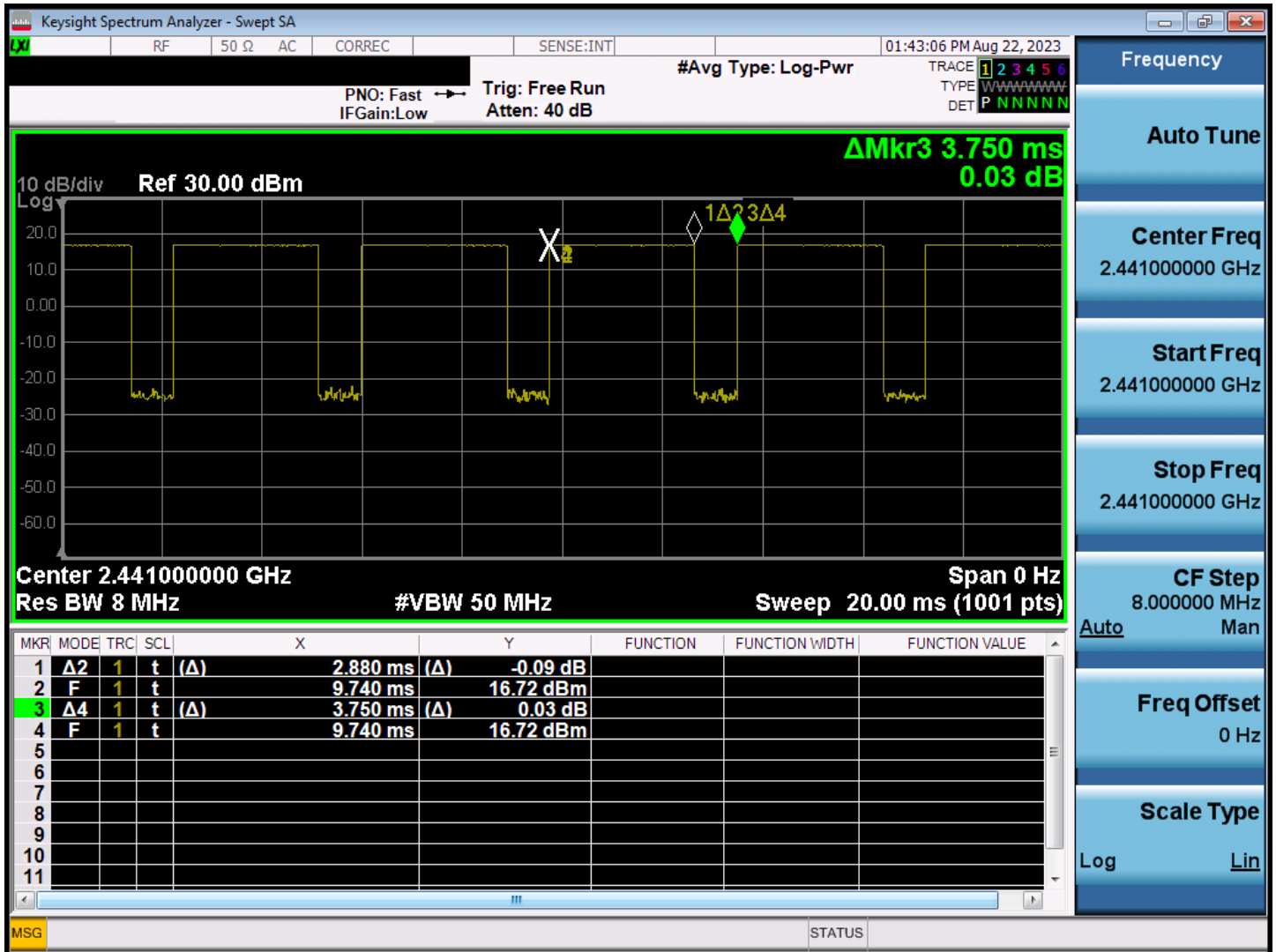
Figure 9.5.1.2 Bluetooth Transmission Plot
