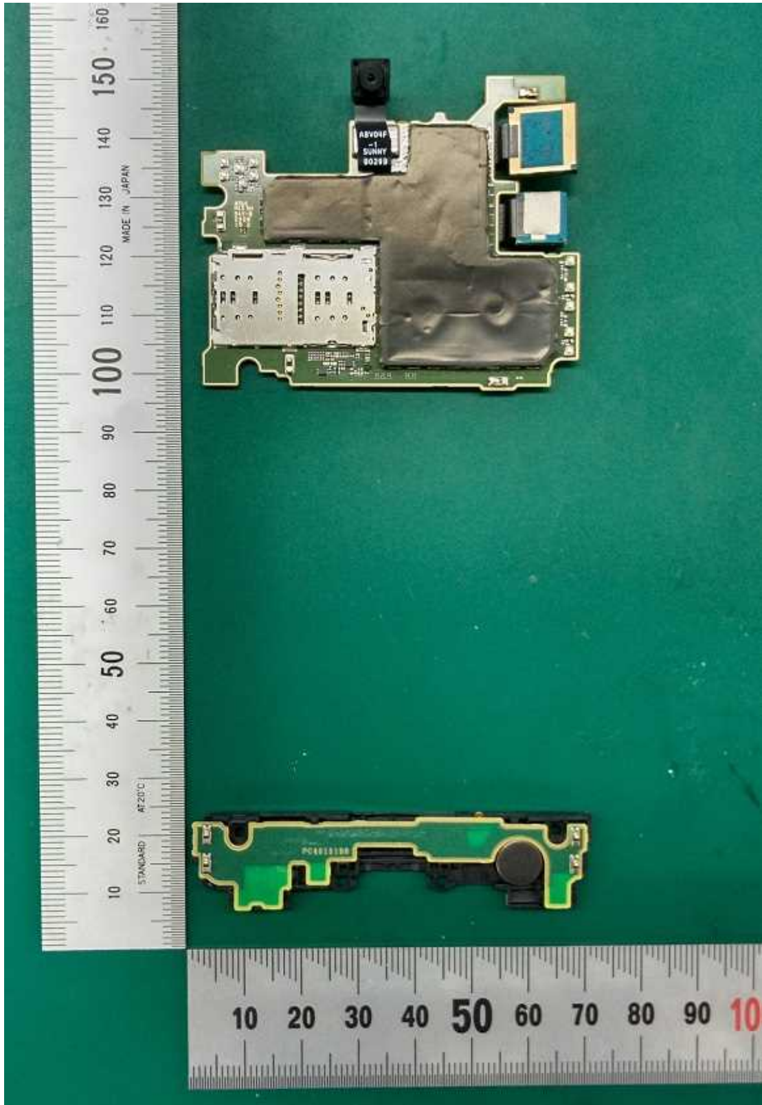
Main PCB, FPC front 1
