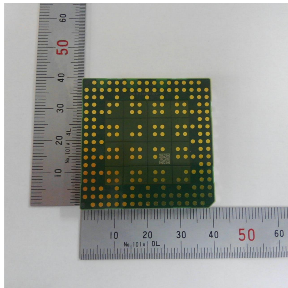
Bottom View
