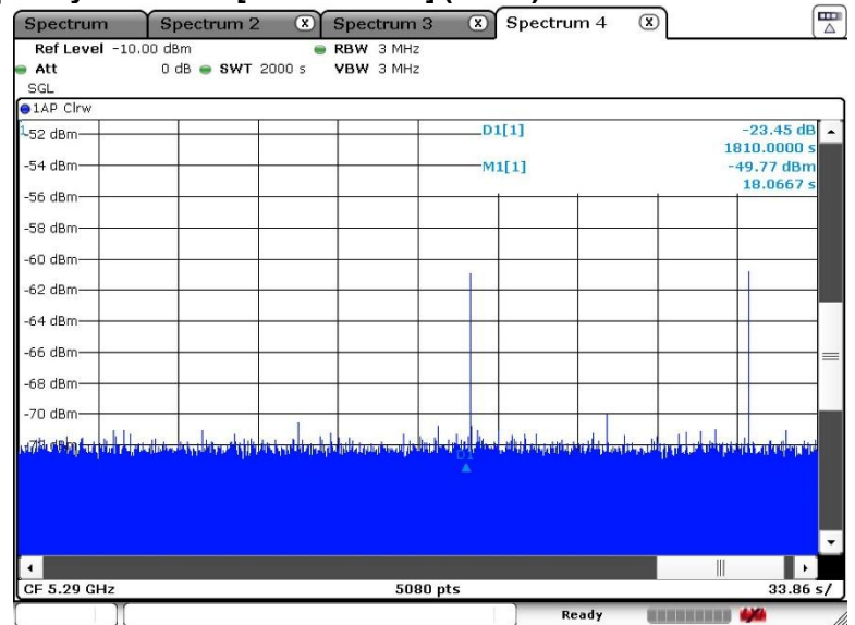
Frequency: 5290MHz [5.3GHz Band] (Zoom)
