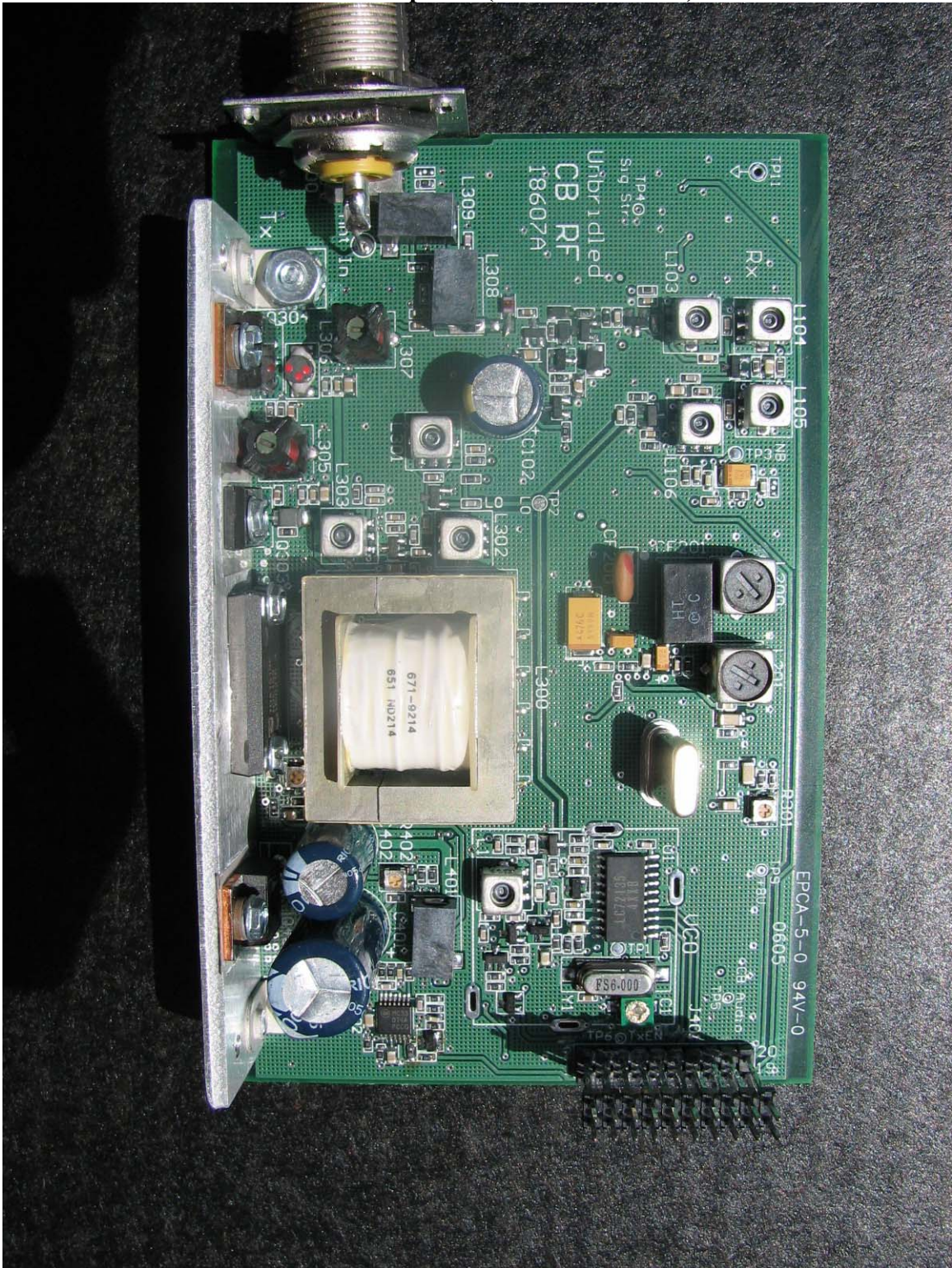
RF Board Top Side (Shields Removed)
