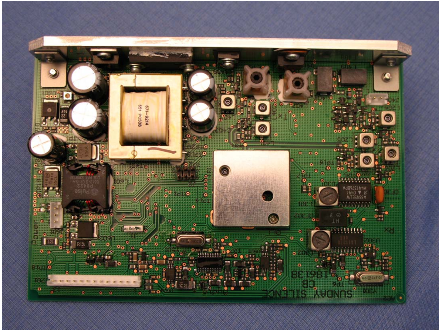
Component Side with Cables Removed
