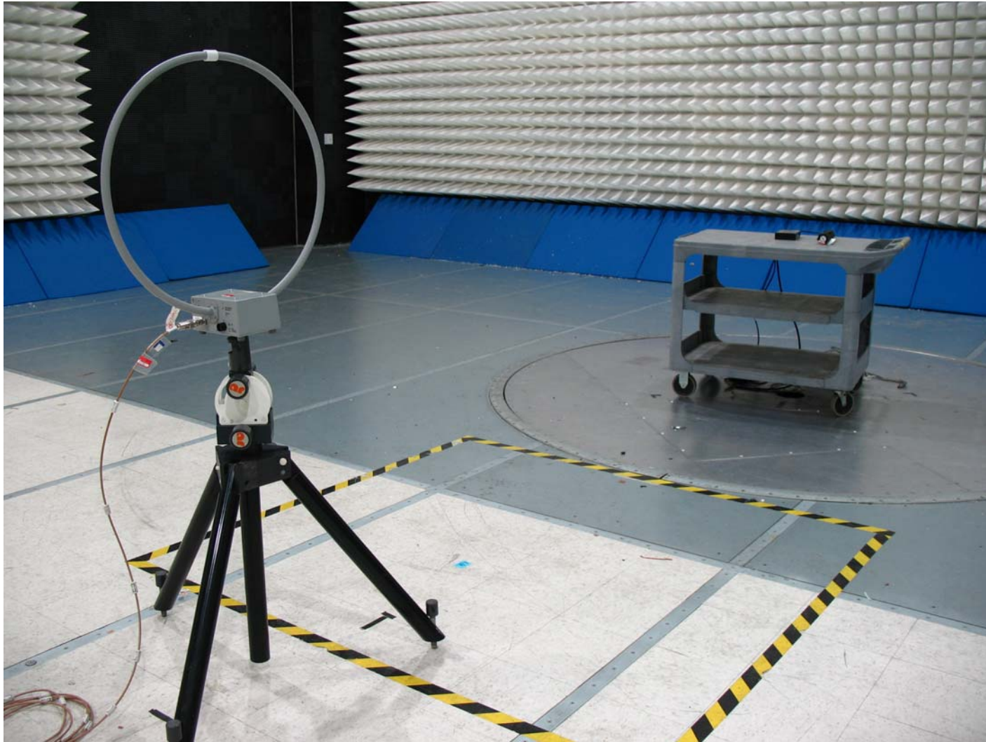
Radiated Testing Below 30MHz Using Magnetic Field Loop Antenna
