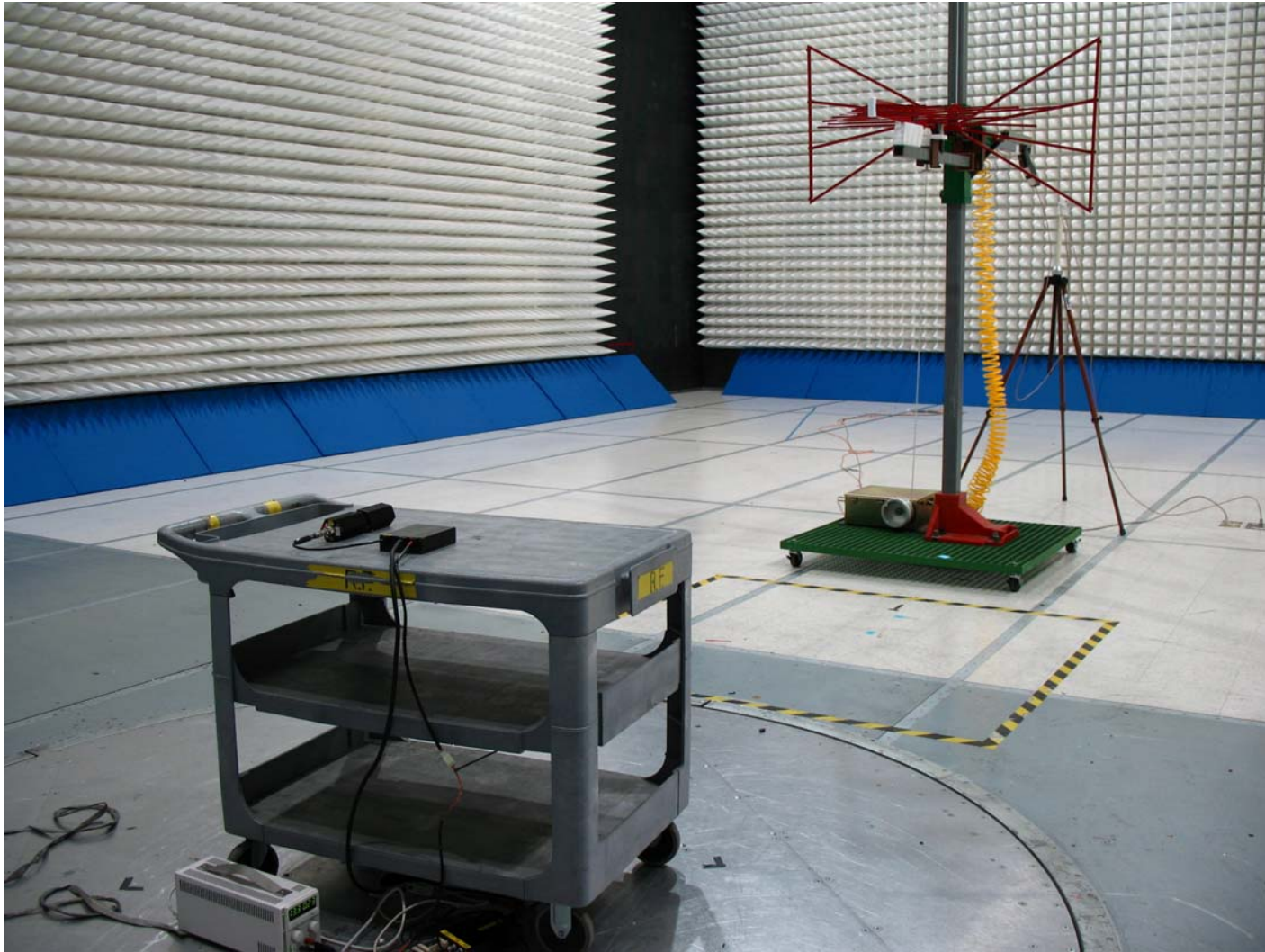
Radiated Testing, Back Side
