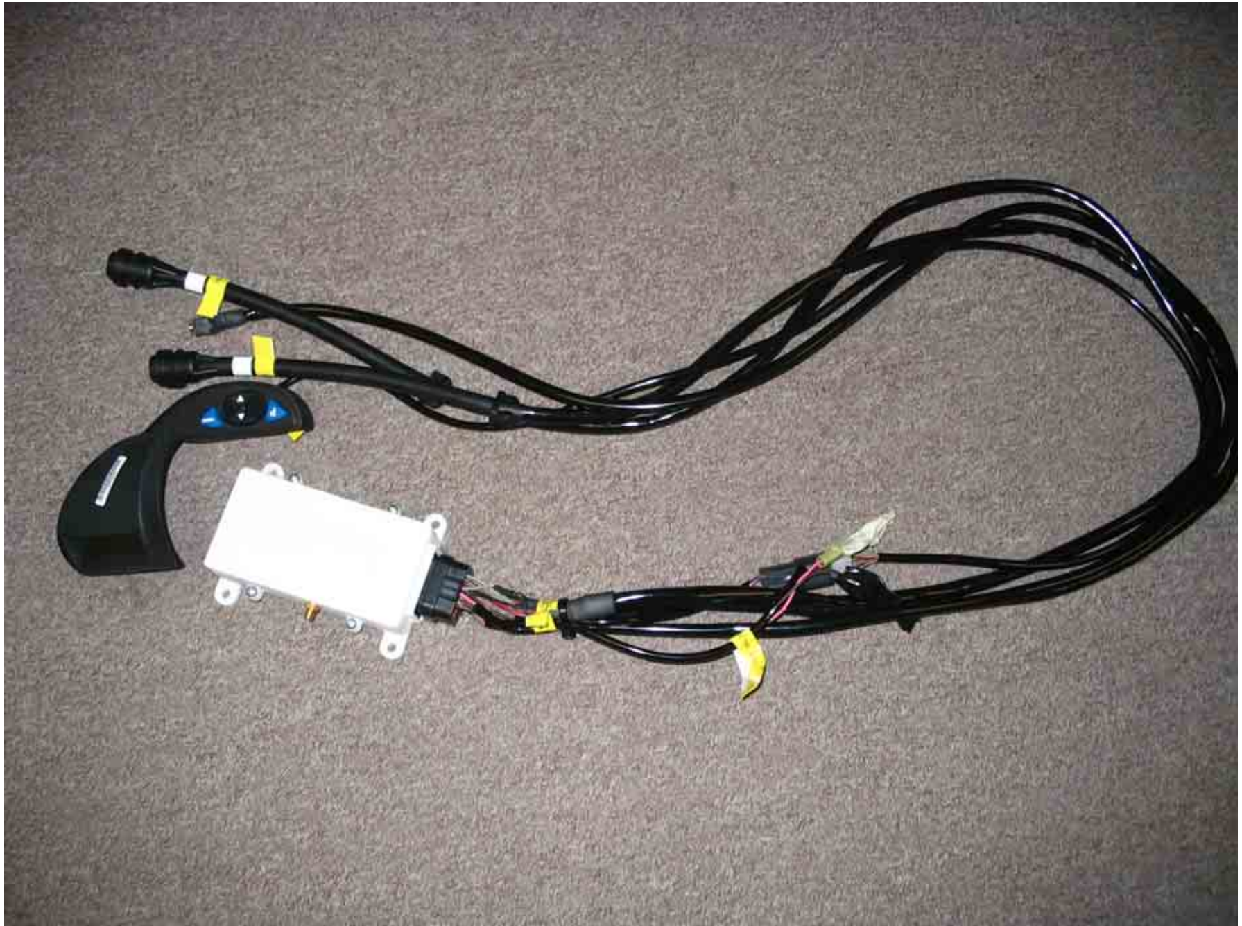
Figure 1: GMSH with Wiring Harness and Handlebar Controls
