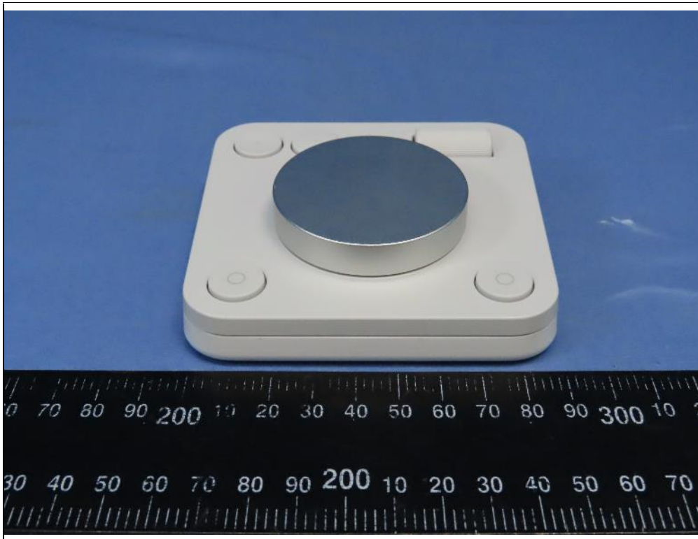
EUT with Magnetic Hall sensor 2 nd Source (PN: MLX90394)
