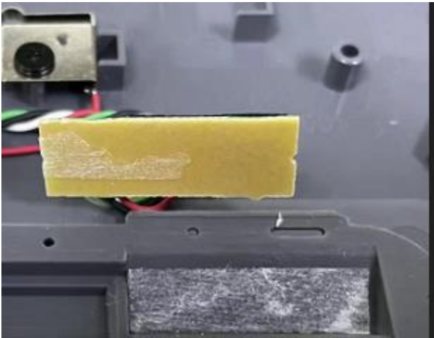
BOARD 2 CLOSE UP BOTTOM
