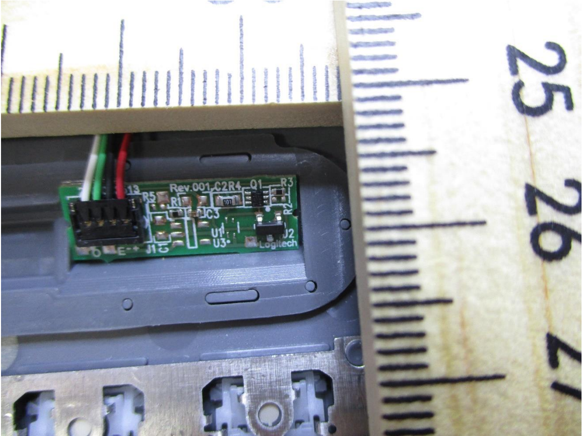
BOARD 2 CLOSE UP TOP
