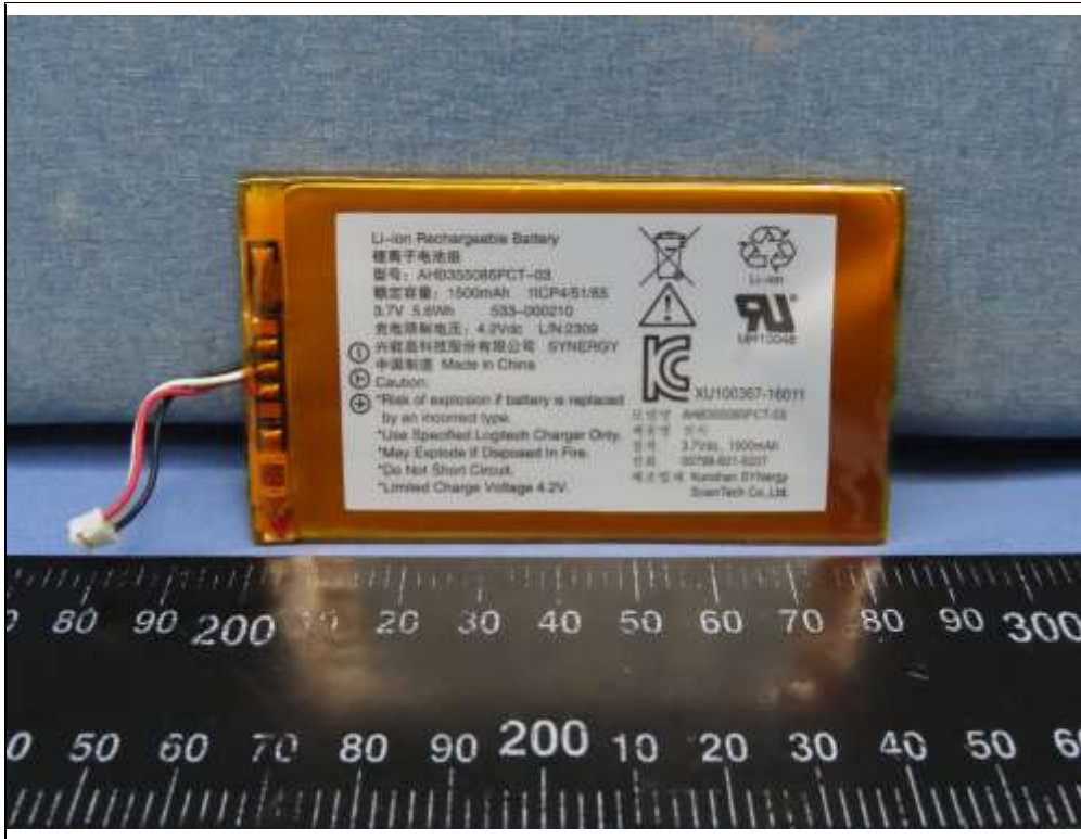
Battery 1 (Model: AHB355085PCT-03 or 533-000210)
