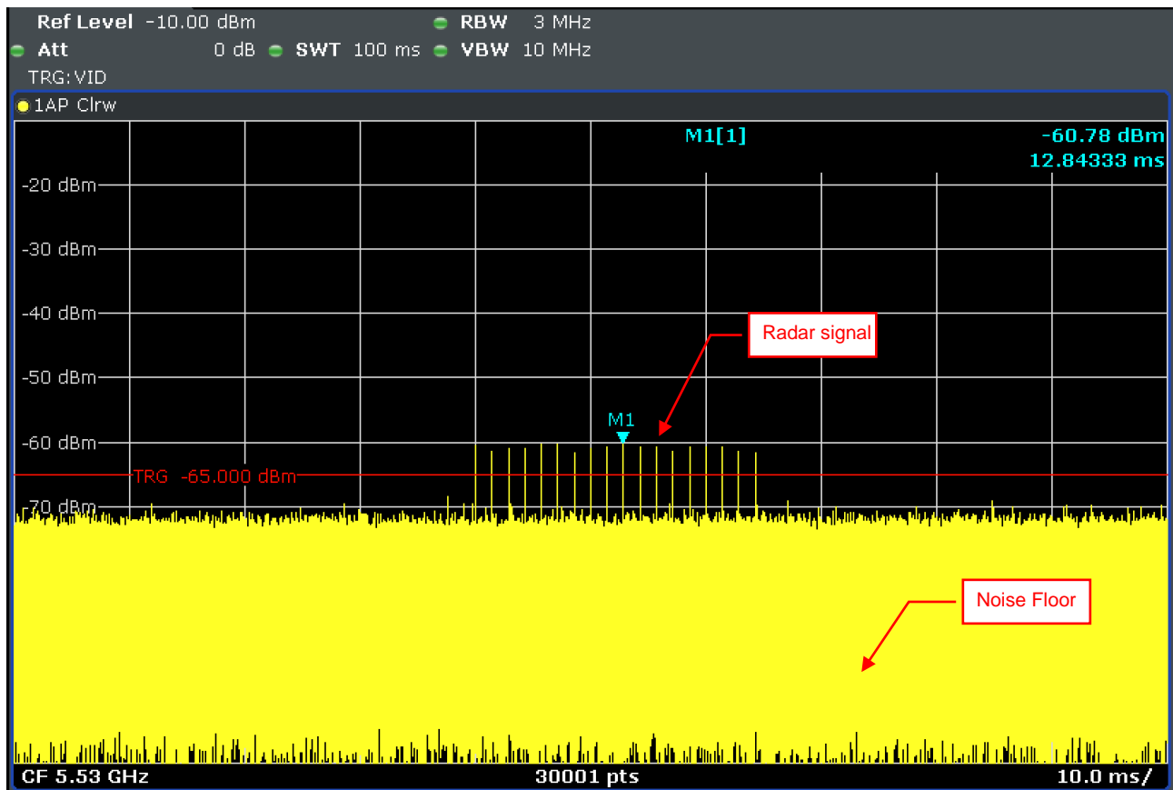
Radar Signal 0
