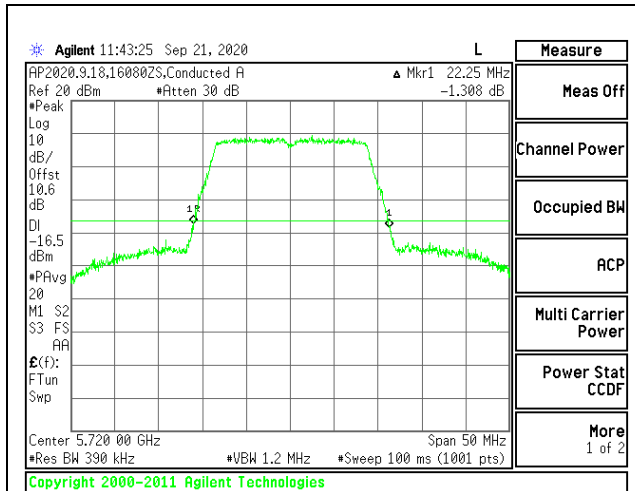
CHANNEL 144 ANTENNA 1
