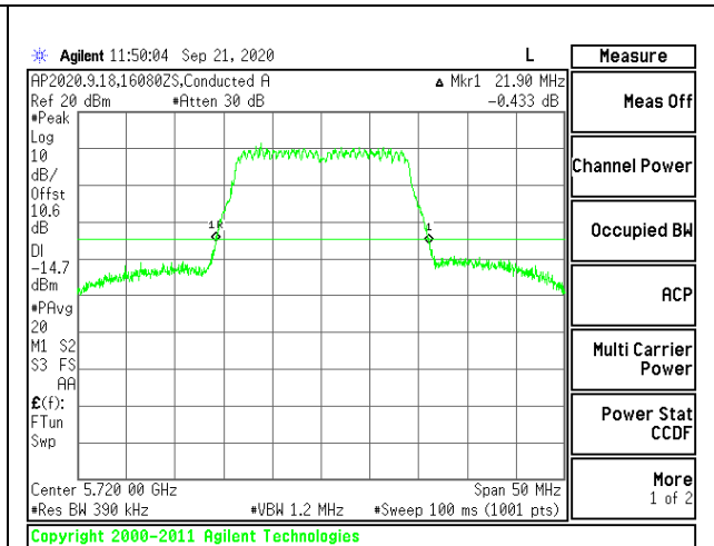
CHANNEL 144 ANTENNA 2
