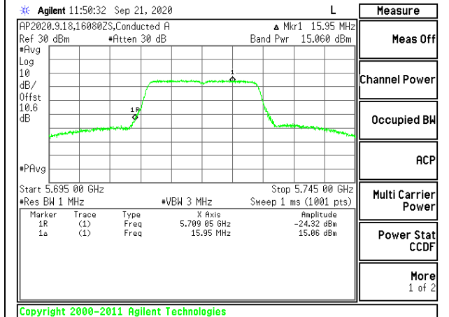
CHANNEL 144 ANTENNA 2 UNII 2-C
