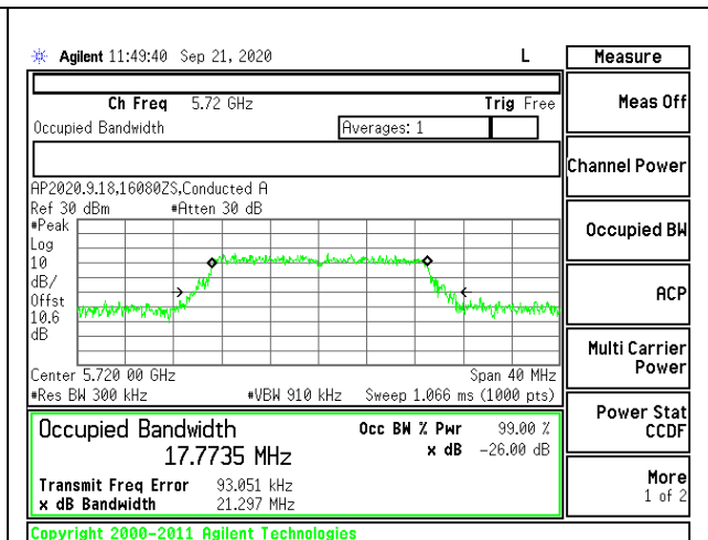
CHANNEL 144 ANTENNA 2
