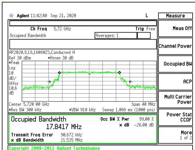
CHANNEL 144 ANTENNA 1
