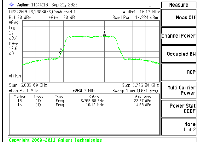
CHANNEL 144 ANTENNA 1 UNII 2-C
