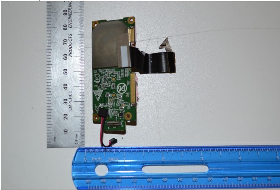
Board 3 top view
