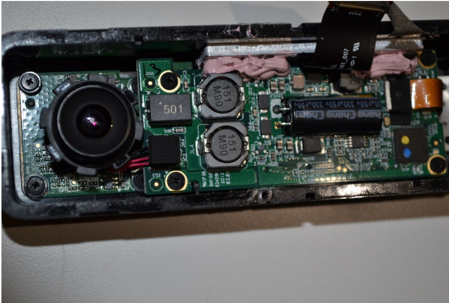
Camera side top close up view
