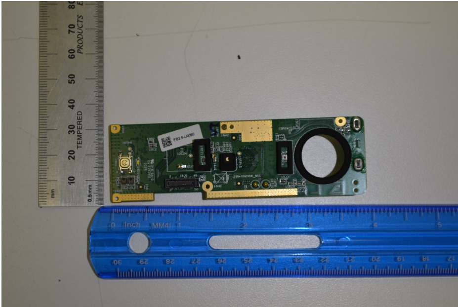
Board 1 bottom view
