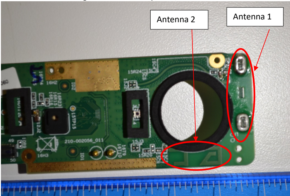
Board 1 radio shielding removed close up view/antennas view
