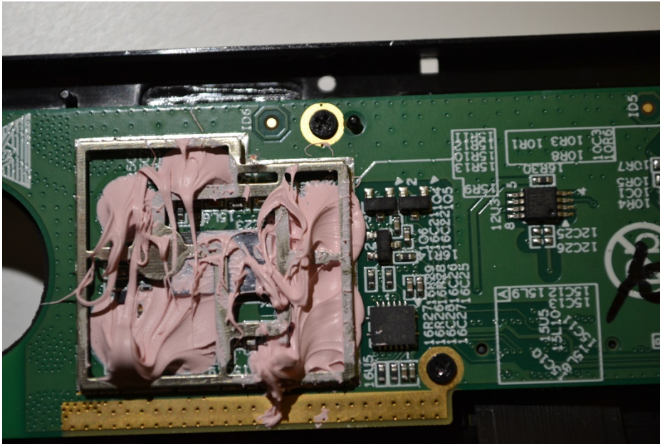
EUT radio shielding removed close up view
