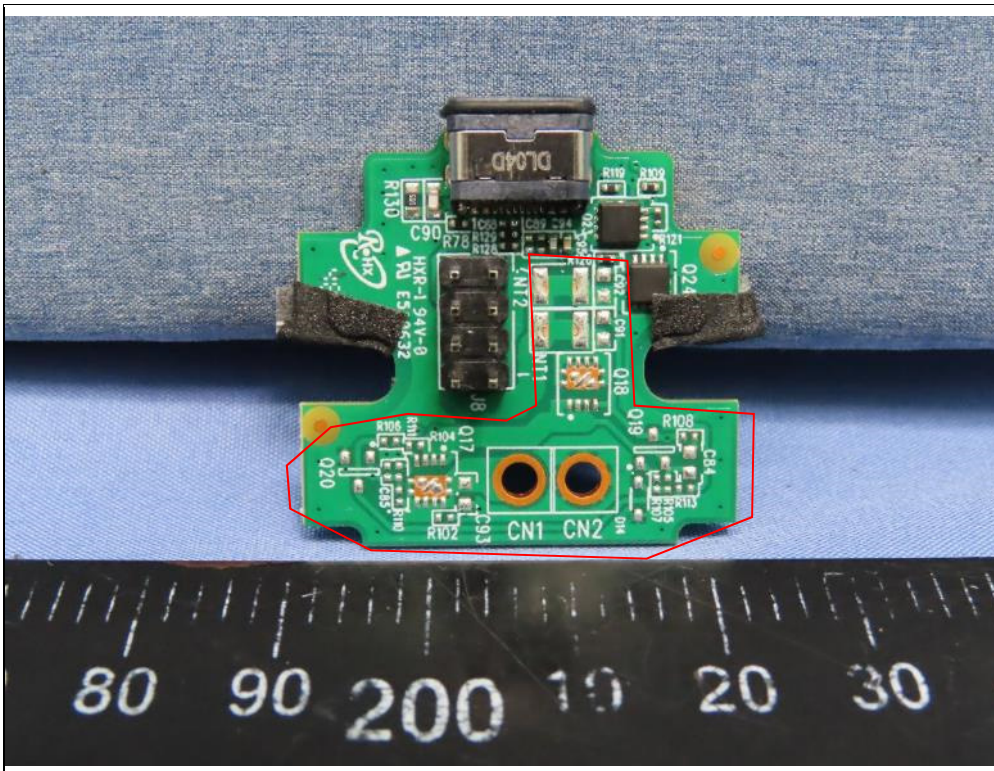
Remove_Charging Dock
