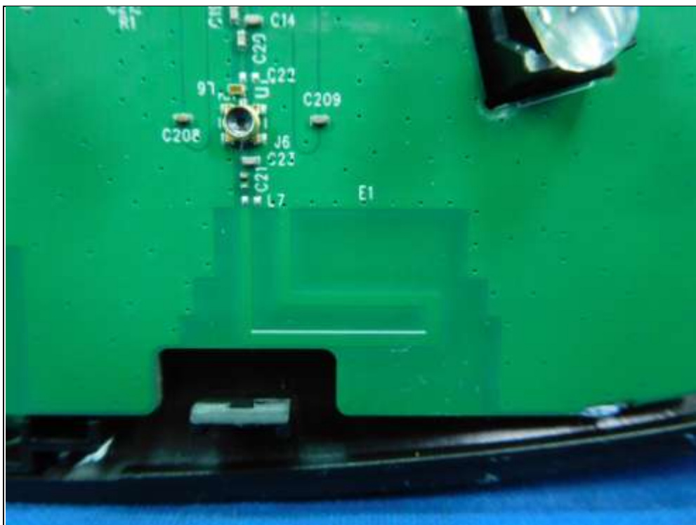
Bluetooth antenna
