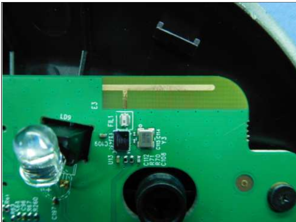
GFSK antenna
