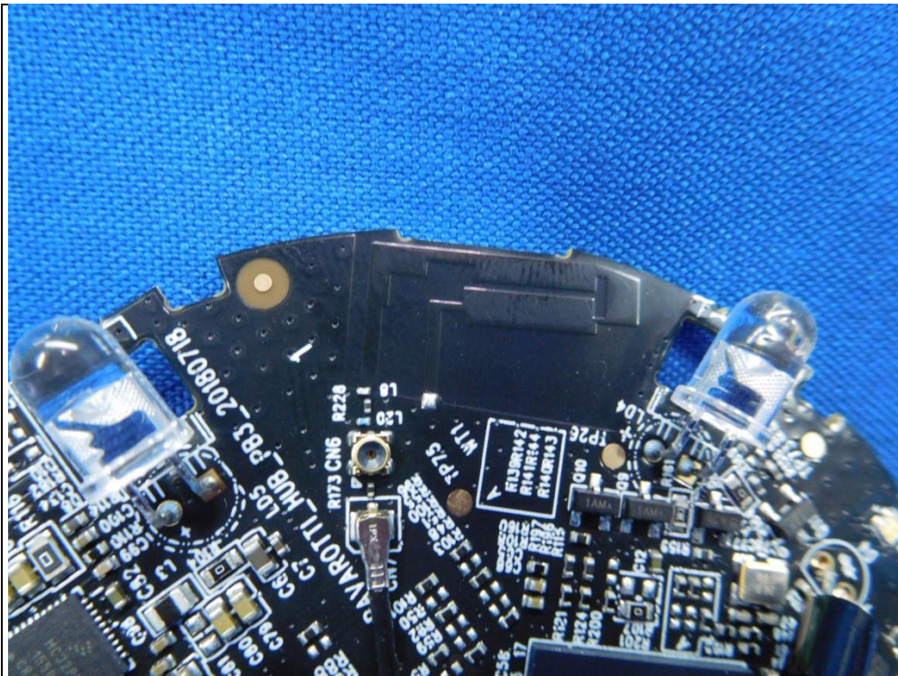
Antenna Chain 1
