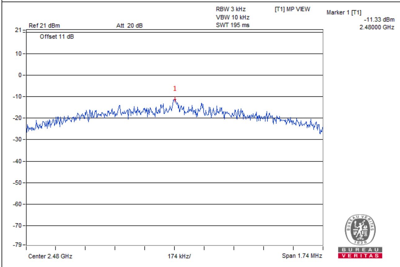
Spectrum Plot of Worst Value CH 79
