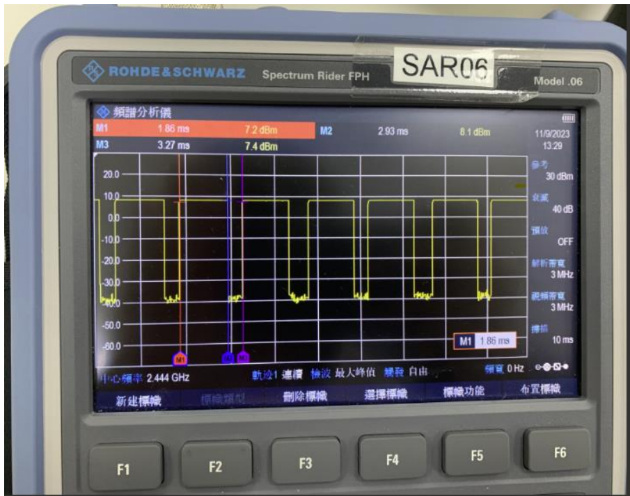
Time-domain plot for SRD transmission signal
