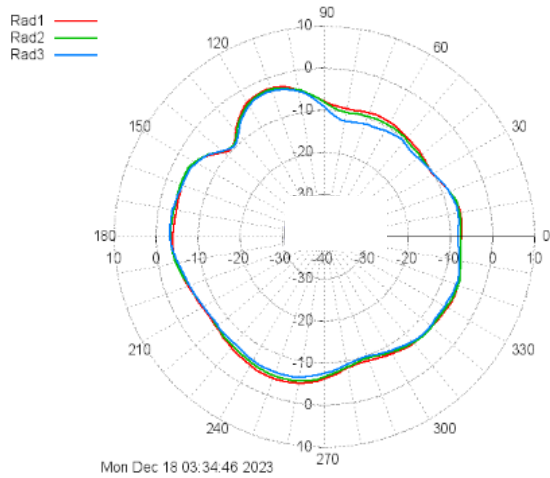
Rad #1: Dagami_RadPatt_Antenna gain_#1_Tx_CH05_V-YZ_0_CORR Rad #2: Dagami_RadPatt_Antenna gain_#1_Tx_CH44_V-YZ_0_CORR Rad #3: Dagami_RadPatt_Antenna gain_#1_Tx_CH74_V-YZ_0_CORR
