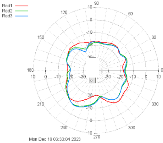
Rad #1: Dagami_RadPatt_Antenna gain_#1_Tx_CH05_V-XZ_0_CORR Rad #2: Dagami_RadPatt_Antenna gain_#1_Tx_CH44_V-XZ_0_CORR Rad #3: Dagami_RadPatt_Antenna gain_#1_Tx_CH74_V-XZ_0_CORR
