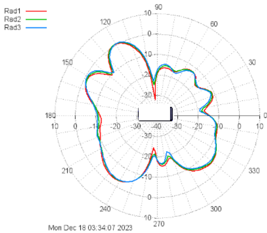
Rad #1: Dagami_RadPatt_Antenna gain_#1_Tx_CH05_H-YZ_0_CORR Rad #2: Dagami_RadPatt_Antenna gain_#1_Tx_CH44_H-YZ_0_CORR Rad #3: Dagami_RadPatt_Antenna gain_#1_Tx_CH74_H-YZ_0_CORR
