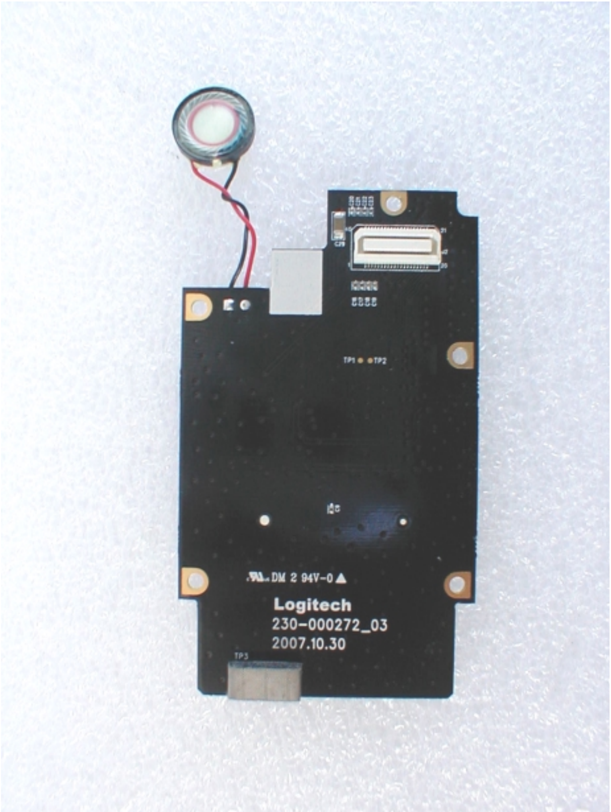
BOTTOM VIEW OF WIRELESS BOARD
