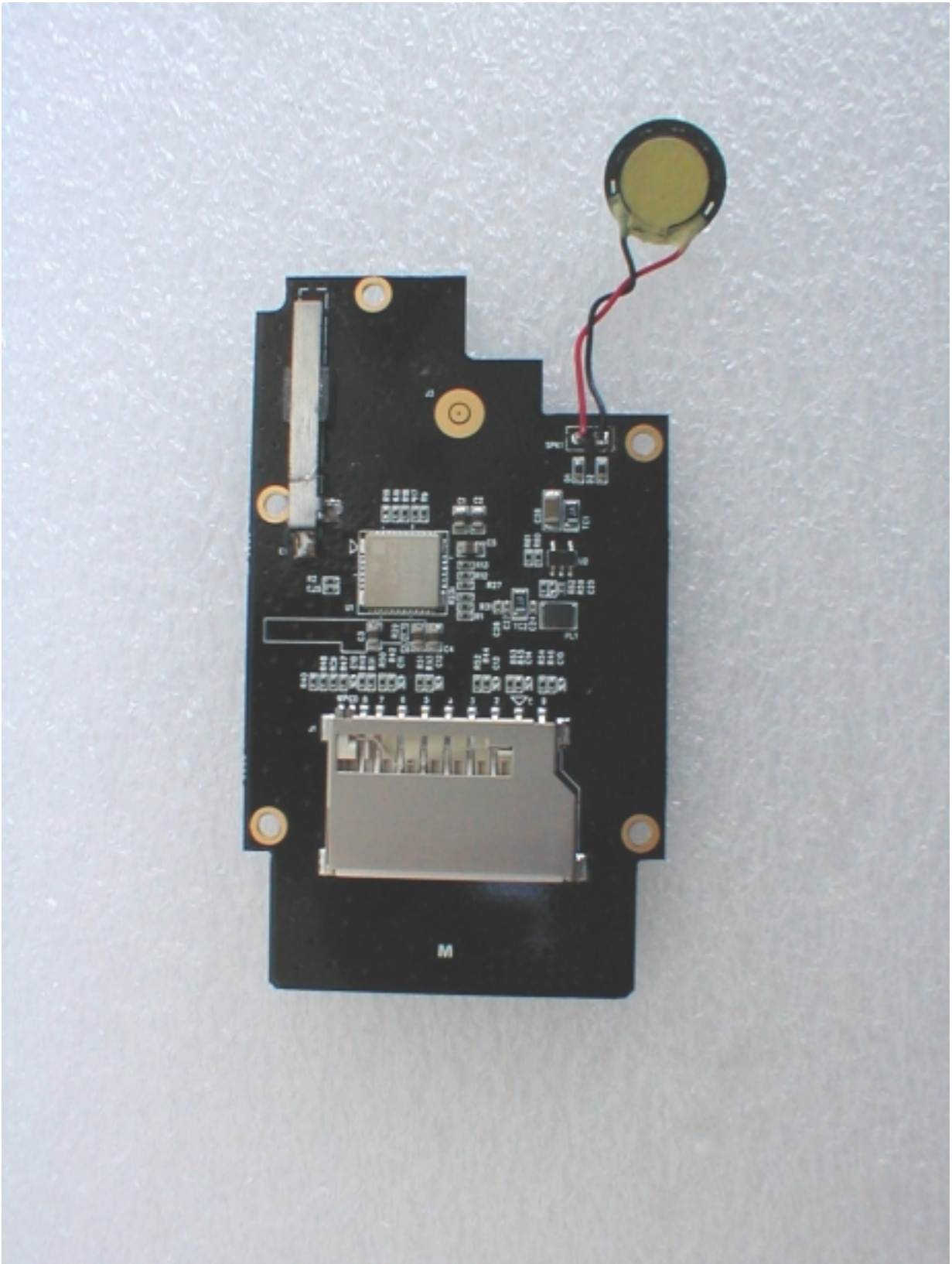
TOP VIEW OF WIRELESS BOARD
