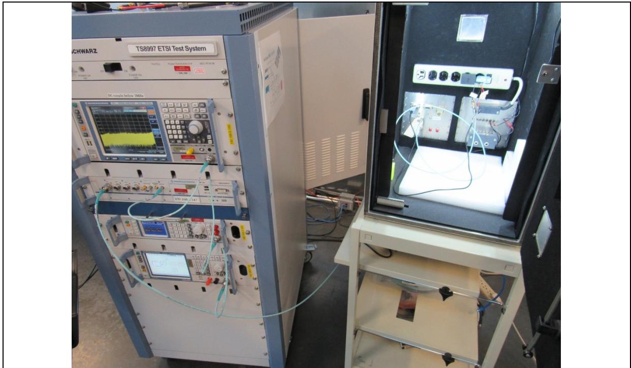
Antenna Port Conducted emissions Setup (Non Spurious Emissions tests)
