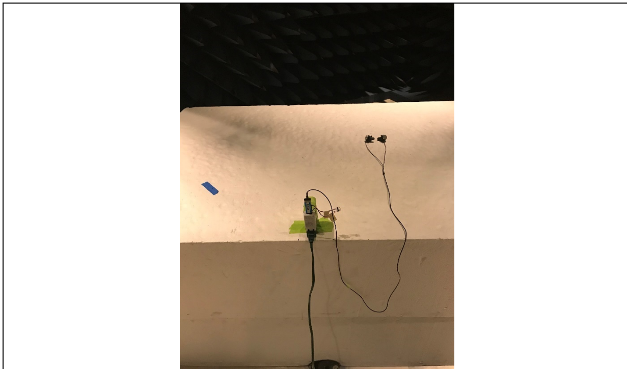
Radiated emissions Setup 30 MHz to 1 GHz (Rear View)
