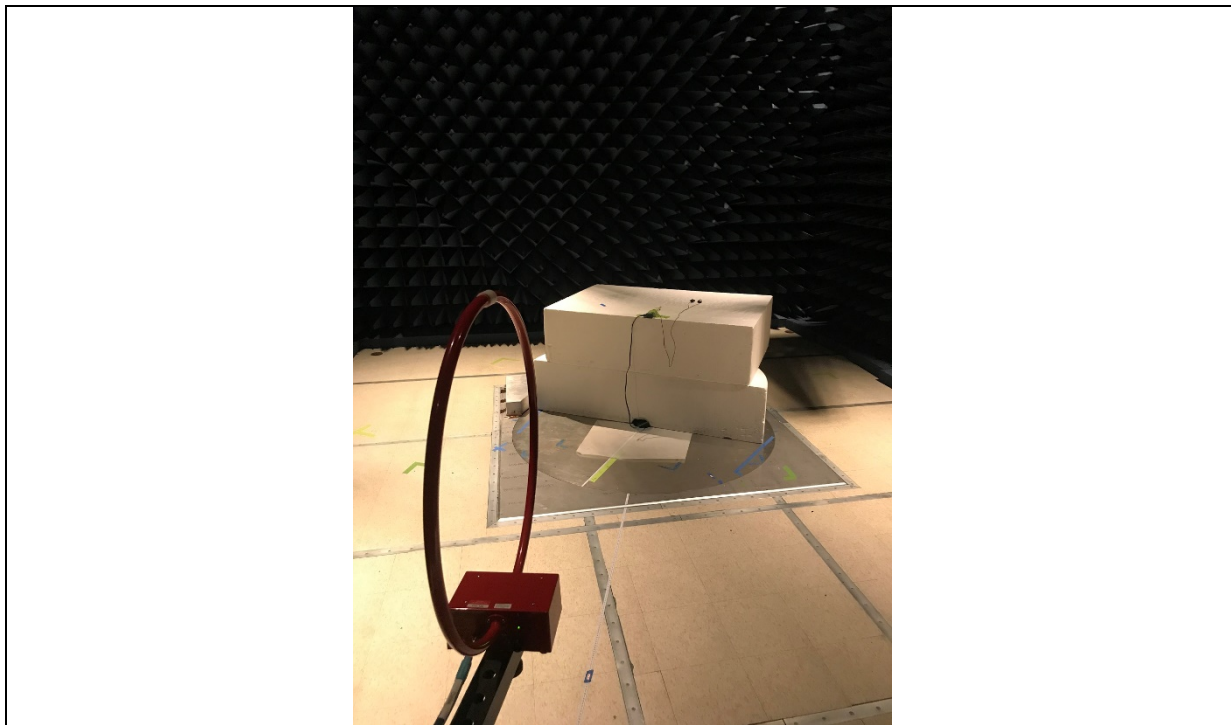
Radiated emissions Setup 9kHz to 30 MHz (Rear View)
