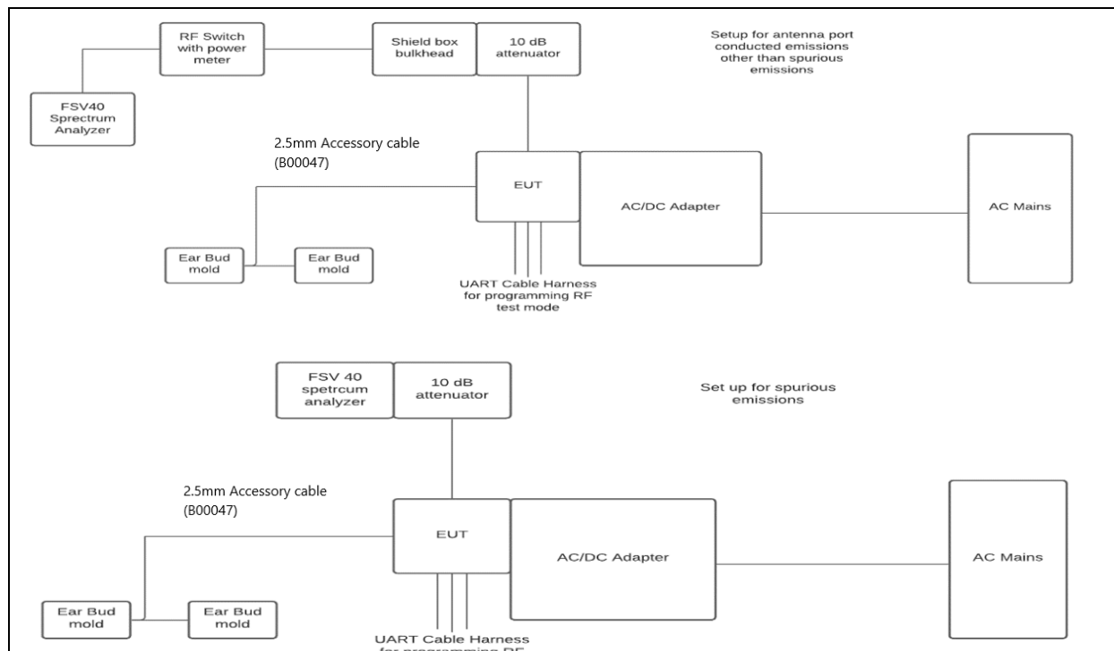
Antenna port conducted emissions Block Diagram of EUT connections
