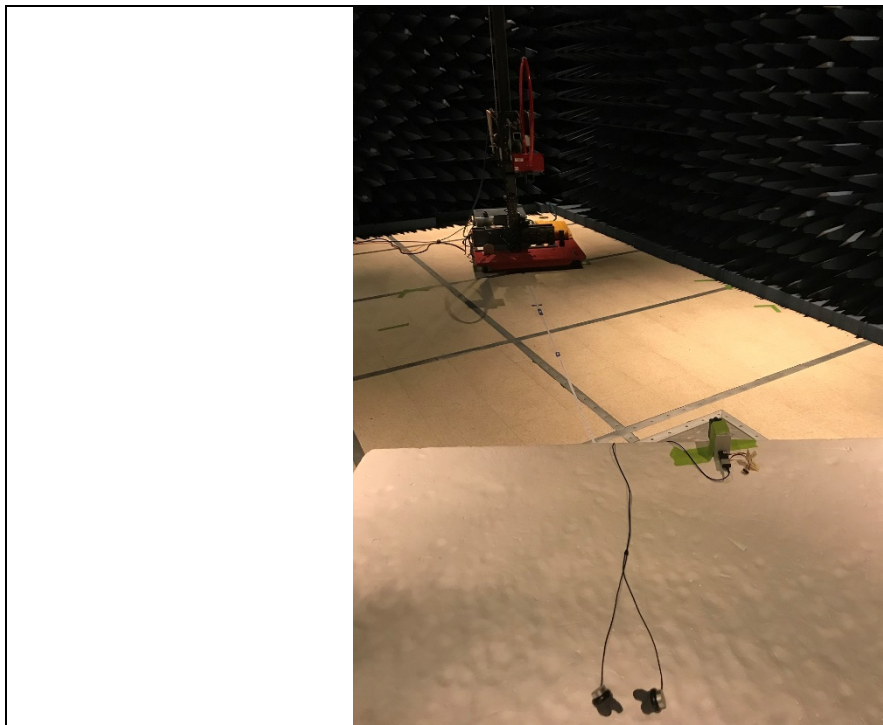
Radiated emissions 9kHz to 30 MHz EUT Setup (Front View)
