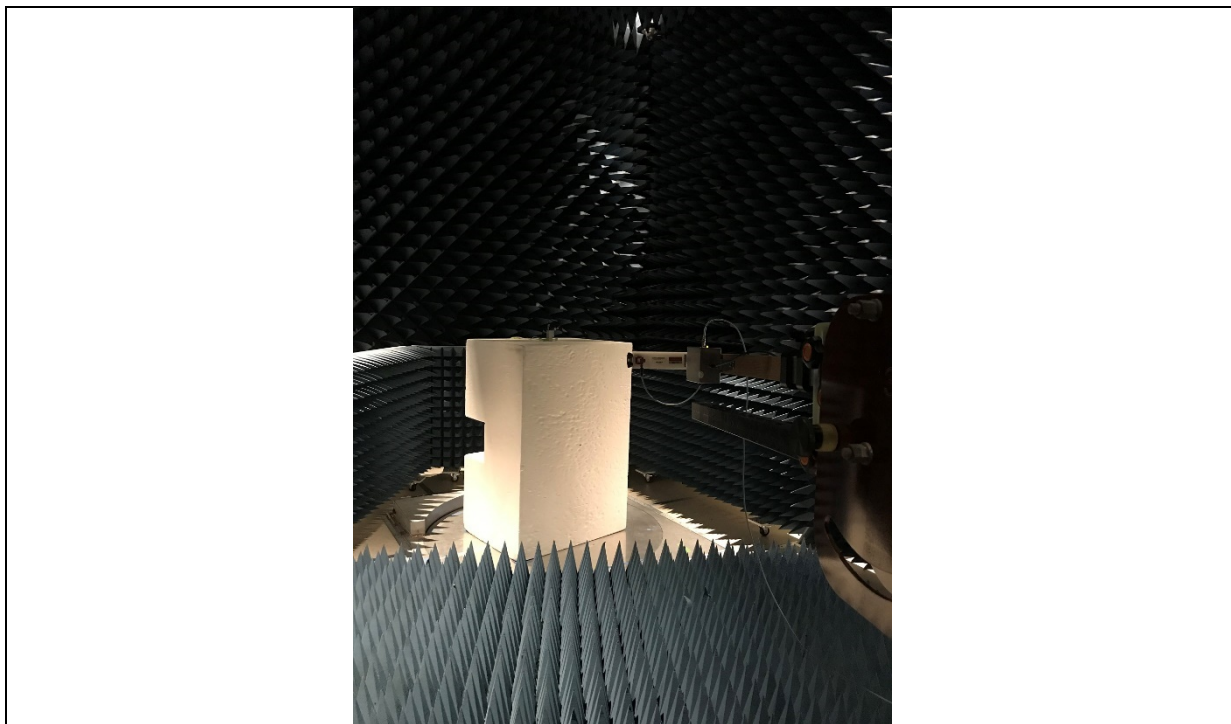
Radiated emissions 18 to 26.5 GHz EUT Setup (Front View)
