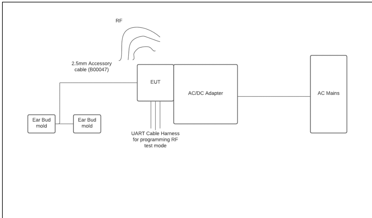
Radiated emissions EUT Block Diagram
