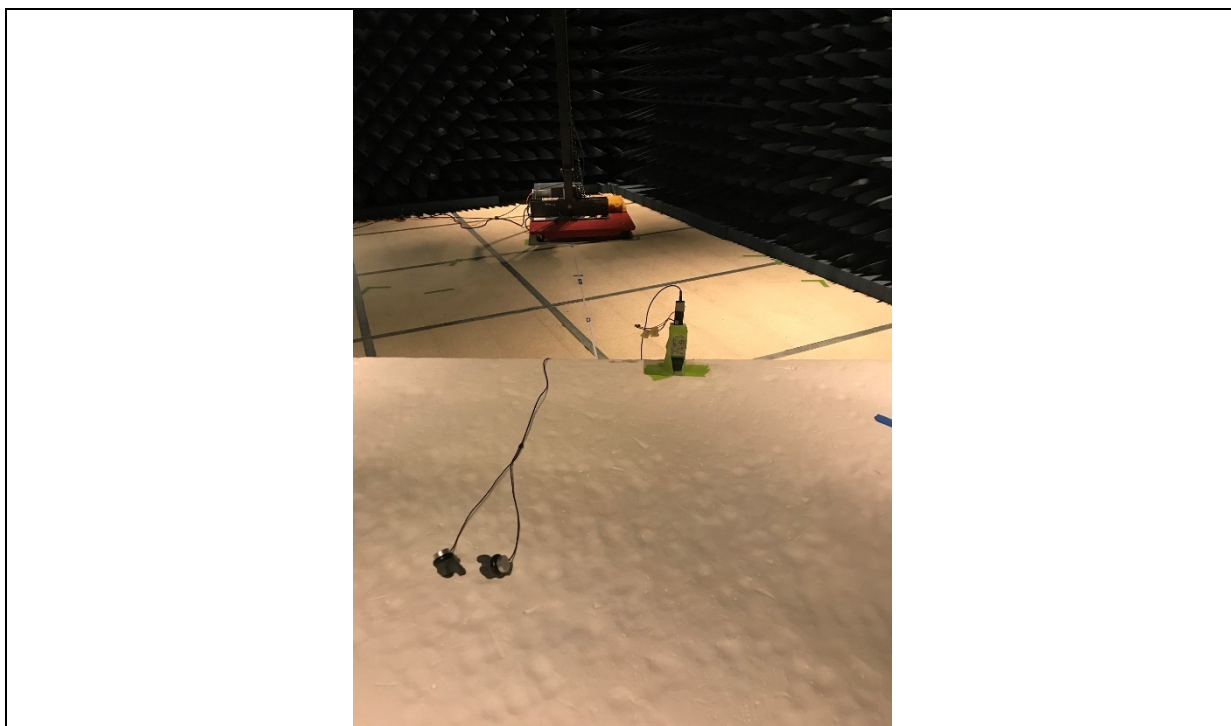
Radiated emissions 30MHz to 1GHz EUT Setup (Front View)
