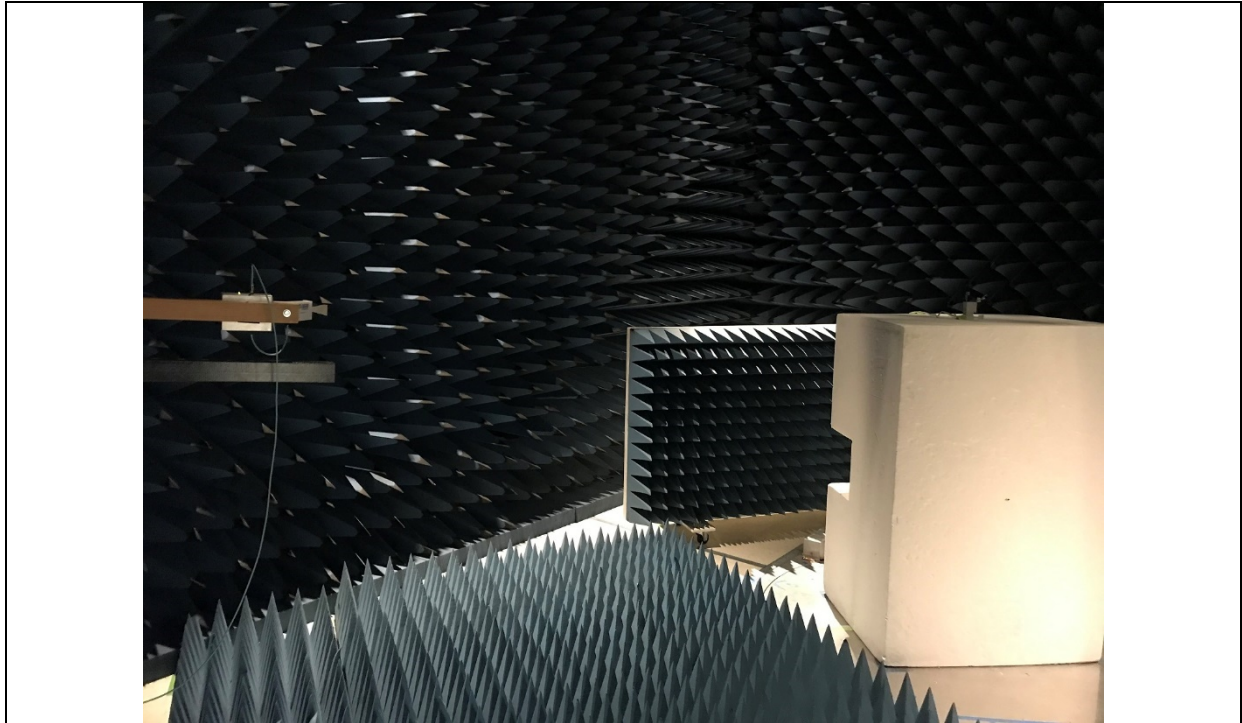
Radiated emissions 1GHz to 18GHz EUT Setup (Overall View)
