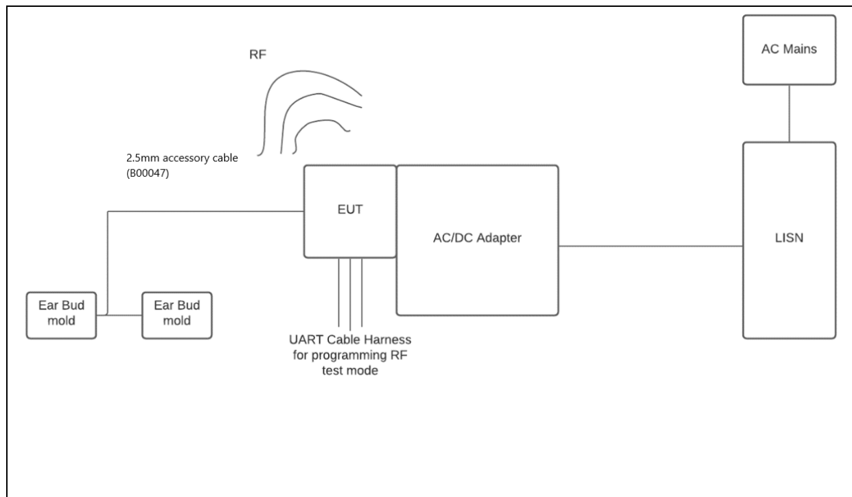
Conducted emissions Block Diagram of EUT connections
